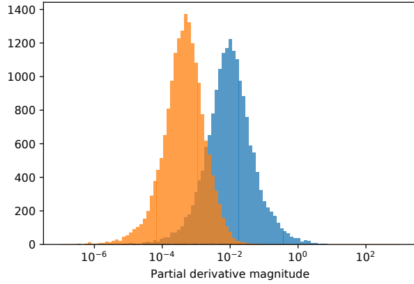
Figure 2: Histograms of the magnitude of the partial derivatives of the loss for the copying memory problem, both at initialization (blue) and after 500 iterations (orange). Note that a few partial derivatives are dominating by a couple of orders of magnitude.
