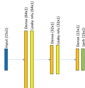
Fig. 3: Generator network.
