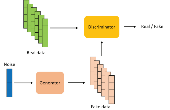
Fig. 1: GAN model for synthetic data generation.
