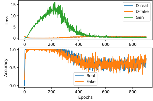
Fig. 5: Line Plots of Loss and Accuracy for a Stable GAN.
