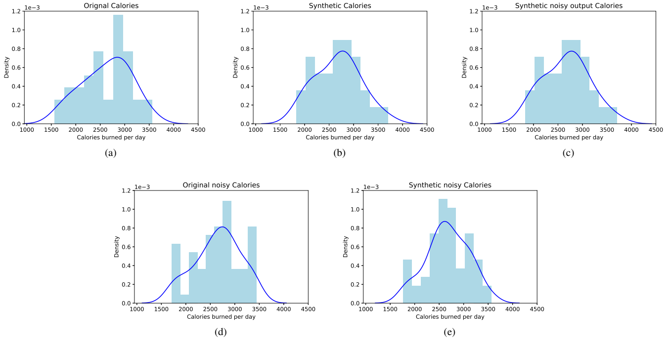
Fig. 6: Histogram distributions for calories burned per day (kcal). Samples: Belgium males with RHR=70–75bpm.
