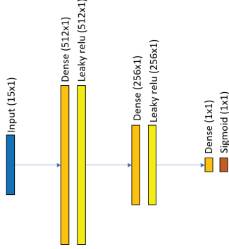
Fig. 4: Discriminator network.
