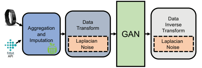
Fig. 2: Data processing pipeline.
