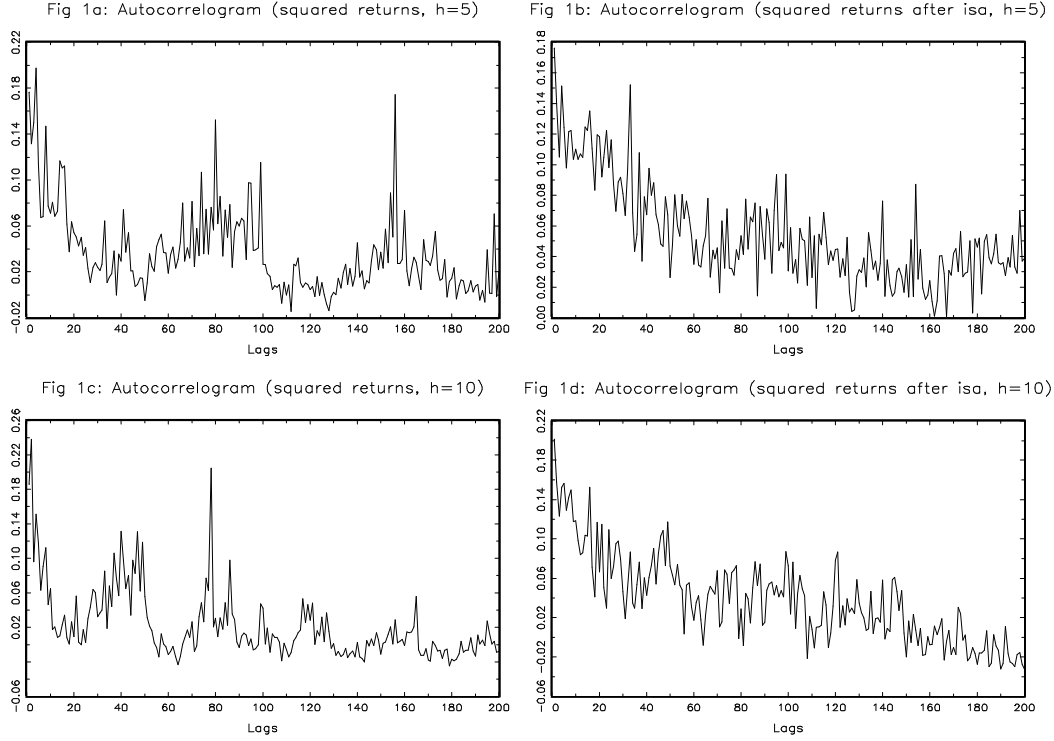
Figure 1: Autocorrelogram for the equidistantly sampled returns ( h=5 and 10 minutes), before (Figures 1a and 1c) and after (Figures 1b and 1d) intraday seasonal adjustment (isa). The returns are defined on the mid-point of the bid-ask quotes of the IBM stock. The period under study is September 96 - November 96 or 13 weeks.
