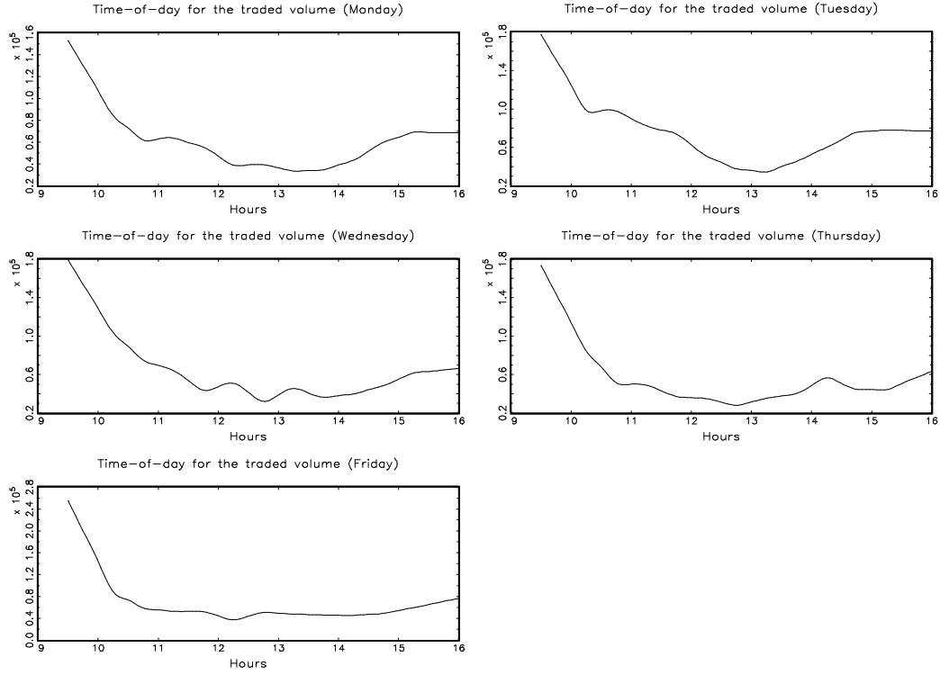
Figure 4: Intraday seasonal component for the traded volume ( h=10 minutes), defined as the total traded volume during 10 minute long intervals.
