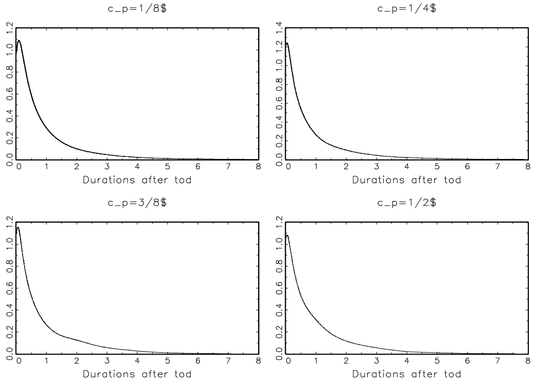
Figure 6: Density functions for the price durations (time-of-day standardized) at the specified threshold c_p . The durations are computed for the IBM stock (September 96 - November 96 or 13 weeks).
