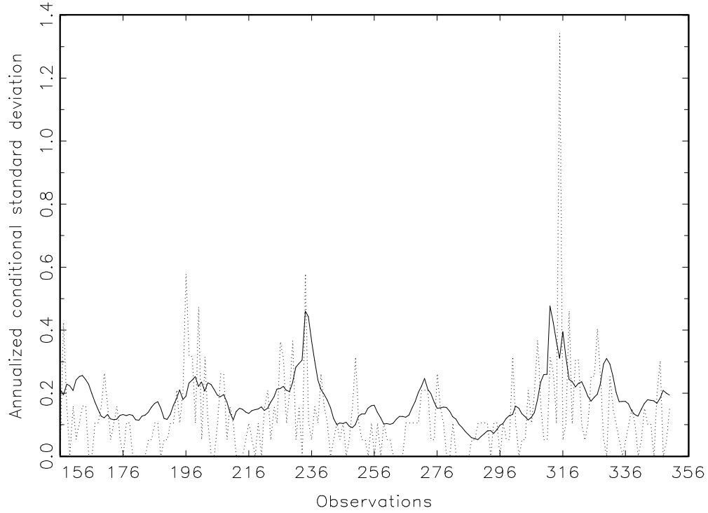
Figure 3: Annualized conditional standard deviation as forecasted by the EGARCH model (continuous line) and observed absolute returns. The returns are defined on the mid-point of the bid-ask quotes of the IBM stock ( h=10 minutes). The model is estimated for the September 96 - October 96 period and the results are plotted for the second week of September.
