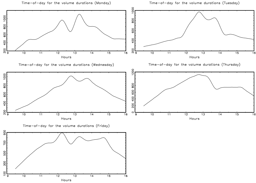
Figure 9: Intraday seasonal component for the volume durations with c_v = 50,000 shares. The durations are computed for the IBM stock (September 96 - November 96 or 13 weeks).
