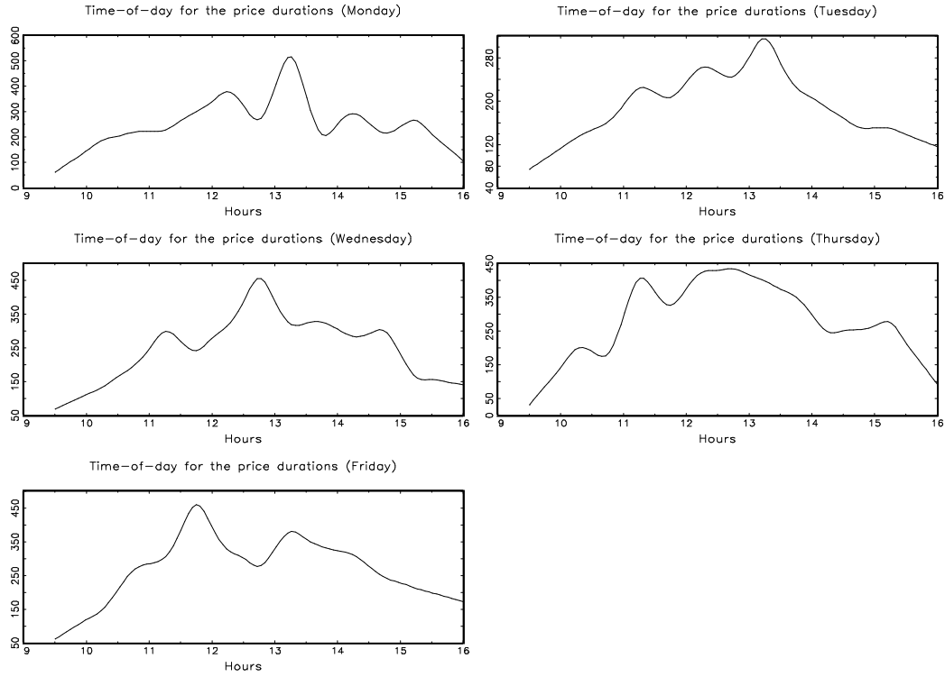
Figure 5: Intraday seasonal component for the price durations with c_p = \frac{1}{8} $. The durations are computed for the IBM stock (September 96 - November 96 or 13 weeks).
