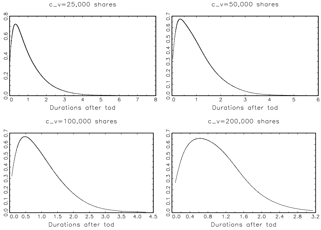
Figure 10: Density functions for the volume durations (time-of-day standardized) at the specified threshold c_v . The durations are computed for the IBM stock (September 96 - November 96 or 13 weeks).
