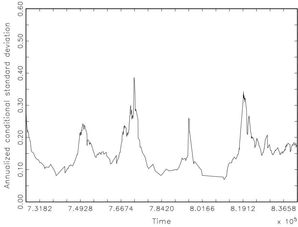
Figure 8: Annualized conditional standard deviation as forecasted by the Log-ACD model estimated on the price durations with c_p = \frac{1}{8} $. The model is estimated for the September 96 - October 96 period and the results are plotted for the second week of September.
