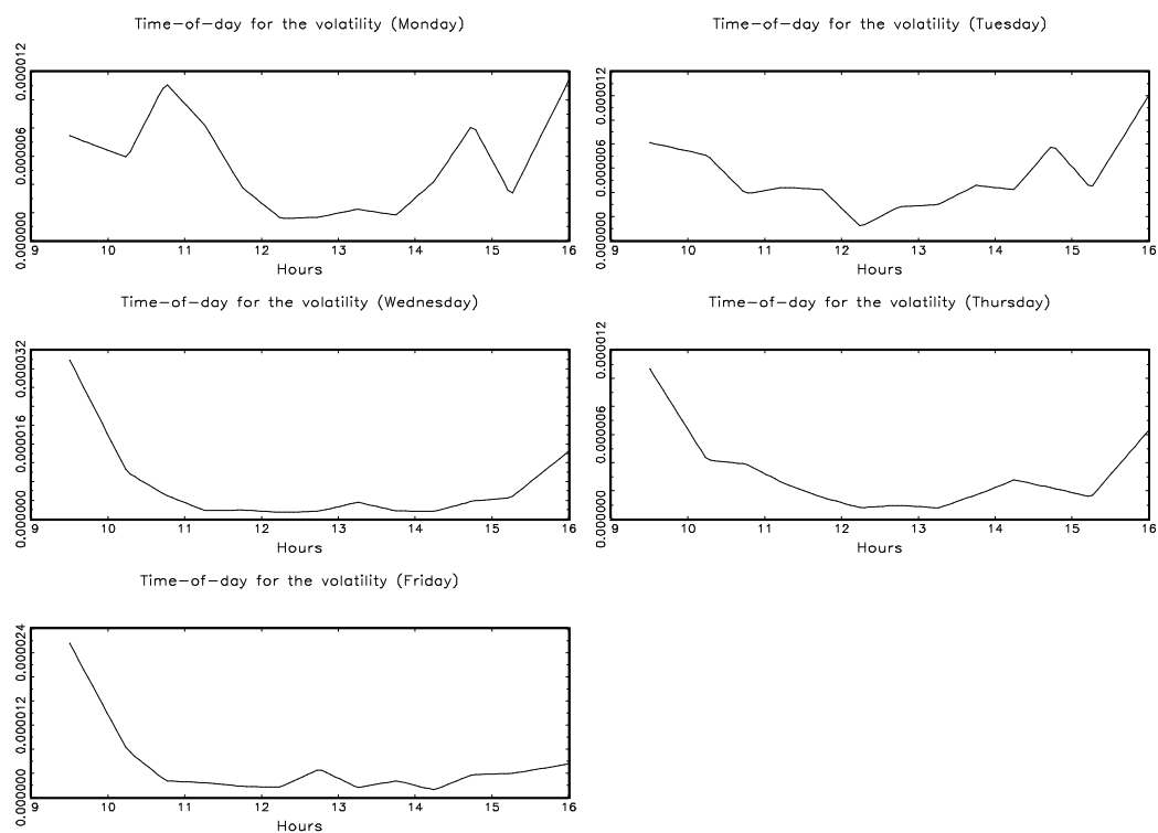
Figure 2: Intraday seasonal component for the volatility computed on equidistantly sampled returns ( h=10 minutes). The returns are defined on the mid-point of the bid-ask quotes of the IBM stock. The period under study is September 96 - November 96 or 13 weeks.
