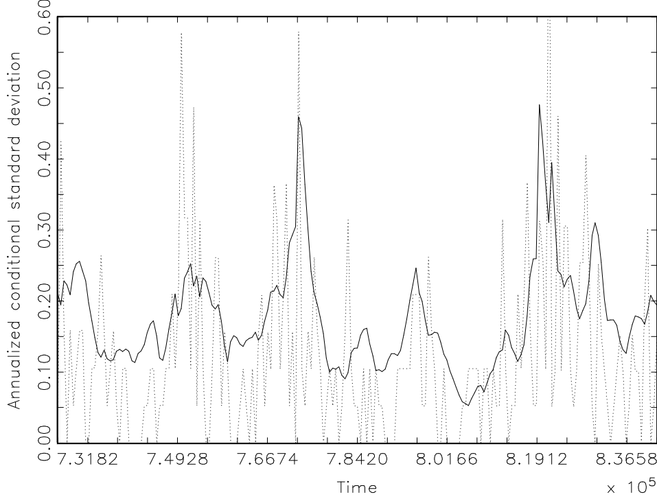
Figure 7: Annualized conditional standard deviation as forecasted by the EGARCH model (continuous line) and observed absolute returns. The returns are defined on the mid-point of the bid-ask quotes of the IBM stock ( h=10 minutes). The model is estimated for the September 96 - October 96 period and the results are plotted for the second week of September.
