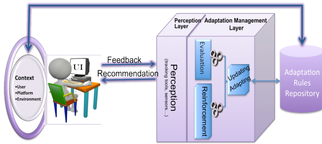
Figure 5. Unified theoretical architecture for adaptation based on machine learning
