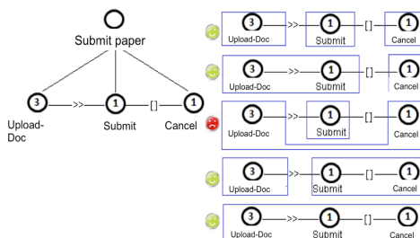
Figure 3. A tasks grouping sample
