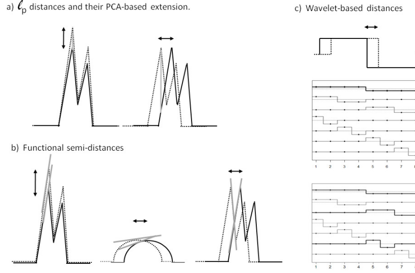
Fig. 1 Schematic illustration of the difficulty for classical methods to take into account horizontal variations of curves. a) l_p distances and PCA-based distances compare curves at each point of measurement, so that patterns that are shifted horizontally are measured distant. An illustrative component of the point-to-point distances is displayed in gray in (a). b) Comparing derivatives, as common functional methods do, allows to overcome that difficulty if the patterns are smooth but fails with sharp shifted patterns. Illustrative derivatives are indicated in light gray in (b). c) Wavelet-based methods capture well the sharp patterns, but their encoding in the basis expansion differs highly if the location of the discontinuity changes a bit: in (c), we illustrate classical Haar-basis expansions of two shifted step function, the only basis vector associated to a non-zero coefficient being highlighted in bold.
