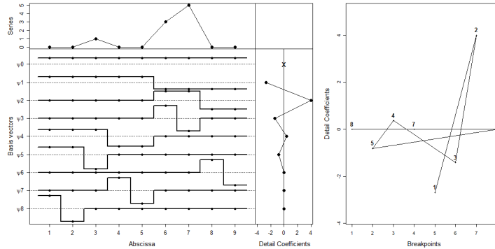
Fig. 2 Left: Illustration of a BUUHW expansion. In the upper part of the figure we plot the series. The corresponding abscissa axis at the very bottom is common for that graph and for the graph of basis vectors. The main part of the figure shows the basis vectors of the Unbalanced Haar wavelet basis that is best suited to the series (BUUHW basis). These vectors are represented rank by rank, as a function of an index along the abscissa axis. Dotted horizontal lines indicate the level zero for each rank. Vertically, from top to bottom on the right hand side, we find the detail coefficients associated with the wavelet expansion. Each coefficient is located next to the corresponding basis vector. For graphical convenience, the value of the coefficient d_0 associated with the constant vector \psi_0 is not indicated. Right: Representation of a series in the b-d plane. The same series is plotted in the plane that is defined by the values of its breakpoints and its detail coefficients. Points are numbered according to their rank in the hierarchy.
