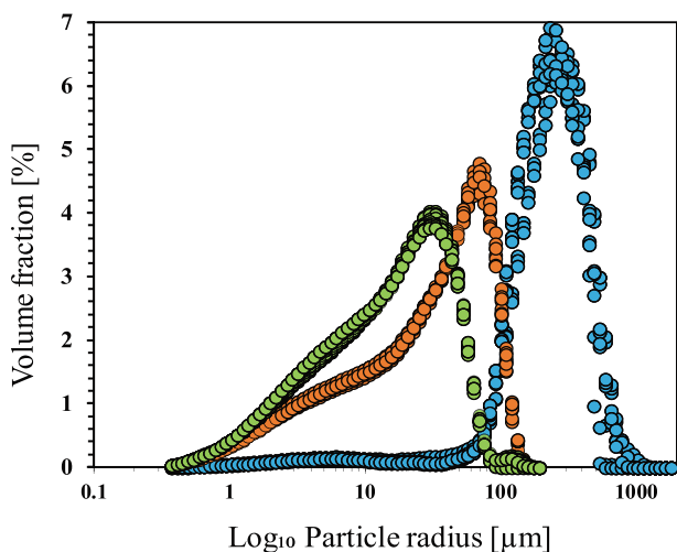
Fig. 1. Particle size distributions of the three sieved populations of rhyolitic glass grains. In shades of green, orange and blue are, respectively, the size distribution ranges <63, 63–90, and ≥90 μm, referred to in the text. We note that indeed, there are particles with radii <63 μm in the 63–90 μm and so these names are simply descriptive of which distribution is used, rather than quantitative. Shown here are 9 measurements for each powder.
