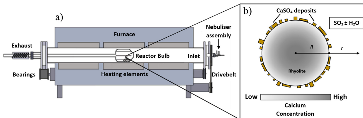
Fig. 2. (a) Schematic of the experimental apparatus, modified from Ayris et al. (2015). The apparatus consists of a split three-heating element tube furnace with a reactor tube inserted into it. At the end of the reactor tube is a bulbous sample holding head which is open at both ends to allow the flux of gas. The whole reactor tube rotates, tumbling particulate samples. Through the furnace assembly, \text{SO}_2 -Ar gas mixtures and nebulized \text{H}_2\text{O} droplets are flushed at known concentrations. (b) A schematic approximation of the process examined in this study showing a spherical rhyolitic glass particle with radius R (radial position r ) that has developed a strong concentration gradient of calcium as \text{CaSO}_4 crystals grow on the surface.
