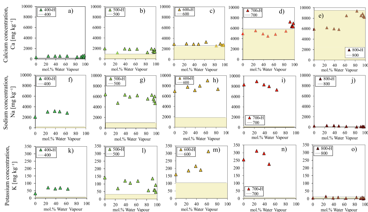
Fig. 6. The effect of water flow rate, converted to mol.% H 2 O, on scavenging processes for (a–e) calcium concentrations, (f–j) sodium concentrations, and (k–o) potassium concentrations. Horizontal lines are the measured value in anhydrous conditions at the same temperature. All samples are the 63–90 µm particle size distribution (Fig. 2) and the exposure time was 60 min in each case.
