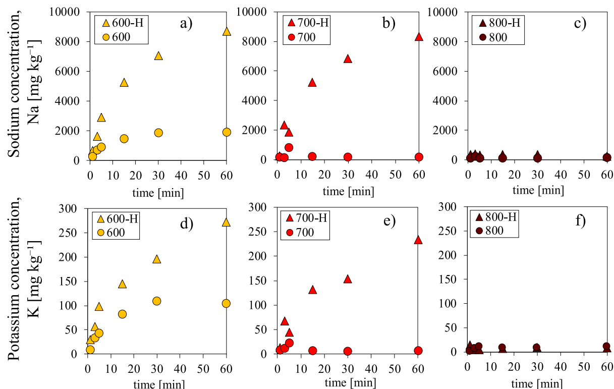
Fig. 7. Direct comparison of the time-dependence of surface concentration in hydrous (62.29 mol.% H 2 O) and anhydrous conditions at 600, 700 and 800 °C for the 63–90 \mu m particle size distribution for (a–c) sodium and (d–f) potassium. We note that calcium does not display significant differences between hydrous and anhydrous conditions (Fig. 6).
