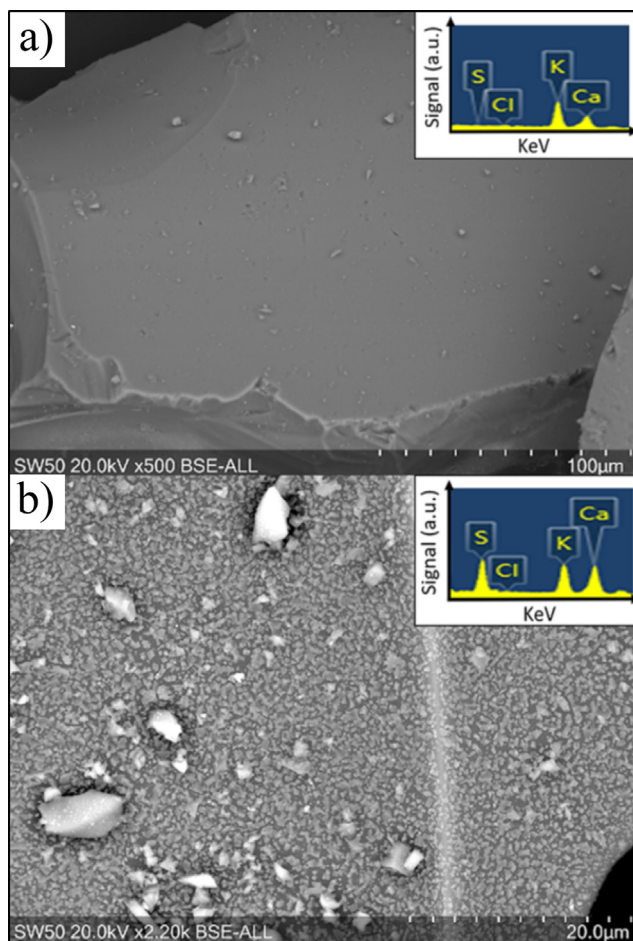
Fig. 3. Scanning electron microscope images of the typical crushed obsidian particles used in this study (a) prior to exposure to gas mixtures at high temperature, and (b) after exposure to \text{SO}_2\text{-Ar} at 800 °C for 60 min. Inset: EDS spectrum of the species of interest S, K, and Ca. Absence of the sulphur peak in (a) the pristine samples suggests sulphur-bearing salt growth occurs due to treatment. Similarly, an increase in the calcium at the post-treated sample spectrum (b), with respect to that of pristine samples (a), suggests higher concentration due calcium diffusion.
