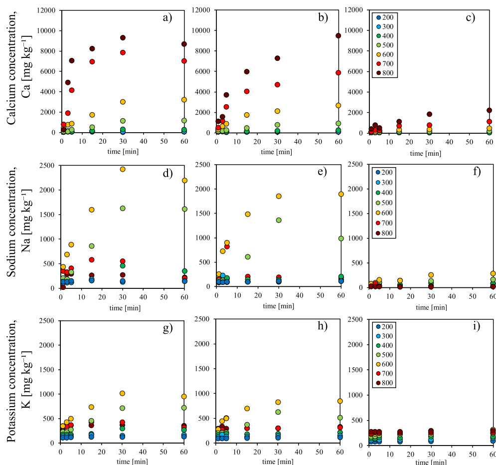
Fig. 4. Raw time-series data for (a–c) \text{Ca}^{2+} , (d–f) \text{Na}^{+} , and (g–i) \text{K}^{+} cation concentrations for a range of temperatures of exposure and for (a), (d) and (g) <63 \mu\text{m} , and for (b), (e) and (h) 63\text{--}90 \mu\text{m} , and for (c), (f) and (i) \geq 90 \mu\text{m} , where the labels in panel (c), (f) and (i) correspond to values of temperature in ^{\circ}\text{C} . We note that for any given time, while high temperatures result in higher values of \text{Ca}^{2+} , this is not true above \sim 600^{\circ}\text{C} for \text{Na}^{+} , or \text{K}^{+} , which is discussed in the main text.
