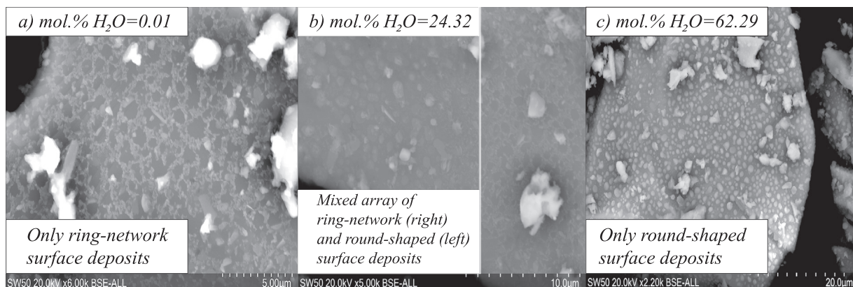
Fig. 5. SEM images of post-experimental sample surfaces treated at 600 °C for 60 minutes and exposed to SO 2 -H 2 O-Ar atmospheres, for three different mol.% H 2 O values.
