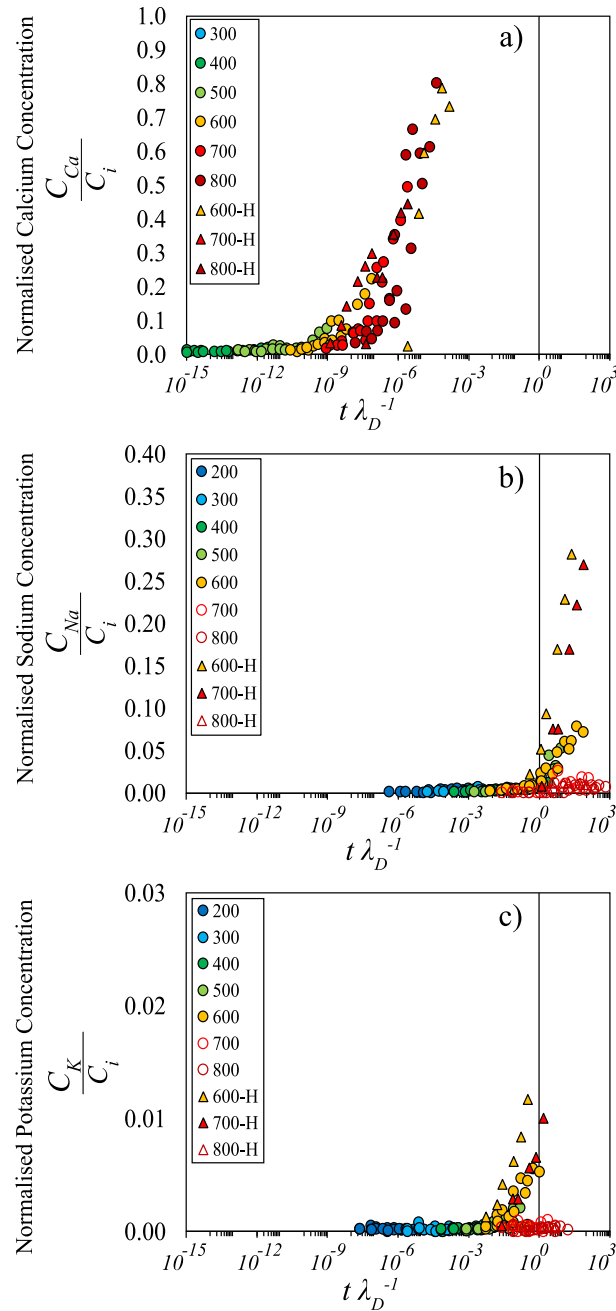
Fig. 8. The concentration of a given cation C_x(t) , i.e., C_{Ca} , C_{Na} , C_K , (a, b and c, respectively) normalized by the initial value of that cation C_i giving \bar{C} = C_x/C_i , as a function of time t normalized by the diffusion time \lambda_D , giving \bar{t} = t/\lambda_D . Using \lambda_D = \langle R \rangle^2/D_x collapses the data over all temperatures and particle size distributions below the critical oxidation temperatures (above which diffusive mass transport to the surface is negligible). Vertical dashed lines simply guide the eye to a normalized time of unity.
