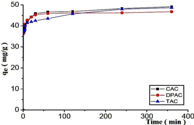
Fig. 4: Kinetic adsorption of orange methyl onto CAC, DPAC and TAC
