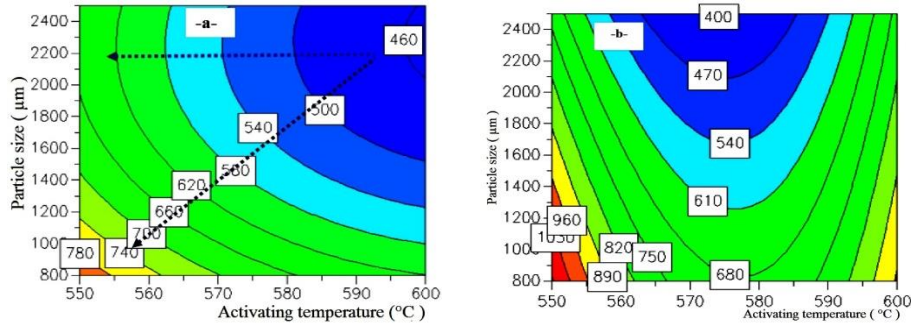
Fig. 3: Iso-response curves for H_3PO_4 – -a- TAC and -b- DPAC
