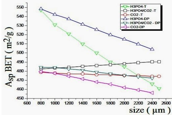
Fig. 2: Effect of particle size on the surface area of (a): TAC and (b): DPAC
