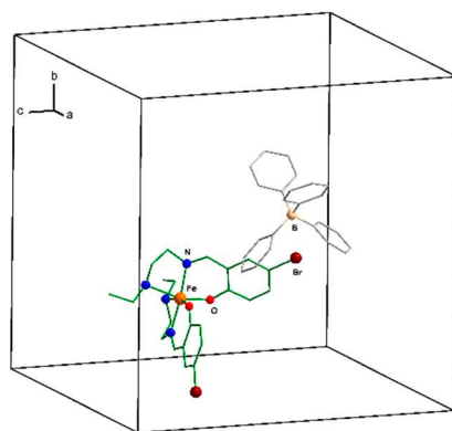
Figure 2. Supercell model of the ion pair [\text{Fe}(\text{5-Br-salEen})_2]\text{BPh}_4 in the LS state.
