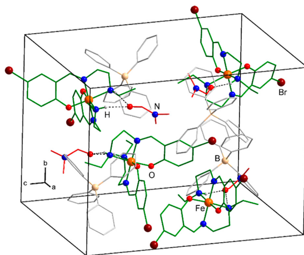
Figure 1. The unit cell of [\text{Fe}(\text{5-Br-salEen})_2]\text{BPh}_4 \cdot \text{DMF} (1) in the LS state. Cationic complex (green) and DMF (red) moieties are highlighted. Hydrogen atoms are omitted for clarity except those involved in internuclear interactions (black dotted). Carbon atoms are represented in the wireframe model. Color code: H—light grey, B—pale pink, N—blue, O—red, Br—dark red, Fe—orange.
