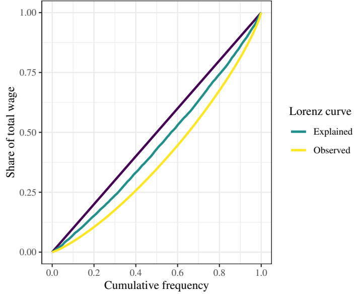
Figure 7: Observed and explained Lorenz curve
