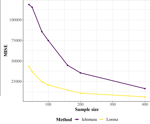
Figure 4: MISE of \hat{H}(X\tau\hat{\theta})
