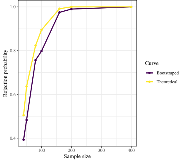
Figure 6: Theoretical and bootstrapped power curves
