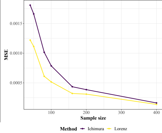
Figure 2: MSE of \widehat{G}_{Y,X}
