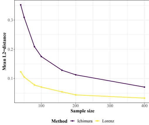
Figure 3: Mean L2-distance between \hat{\theta} and \theta_0
