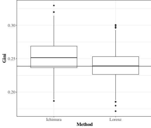
Figure 1: Distribution of \widehat{G}_{Y,X}
