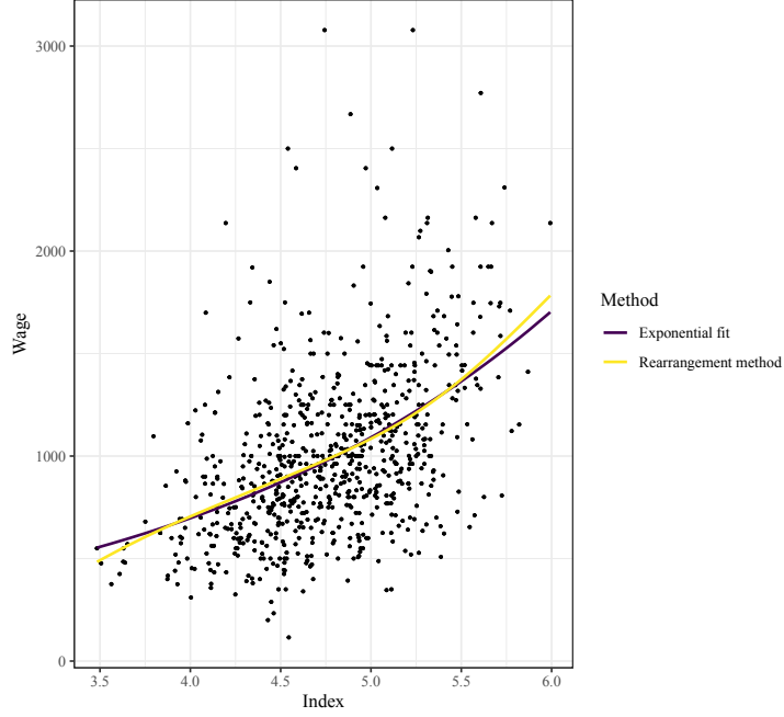
Figure 8: Nonparametric and parametric fit of the wage equation
