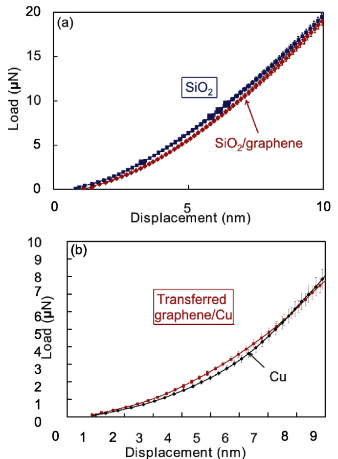
Fig. 5. Load-displacement curves: (a) experimental measurements for SiO 2 and SiO 2 /graphene, and (b) experimental measurements for bare Cu and Cu/graphene (transferred). (A colour version of this figure can be viewed online.)
