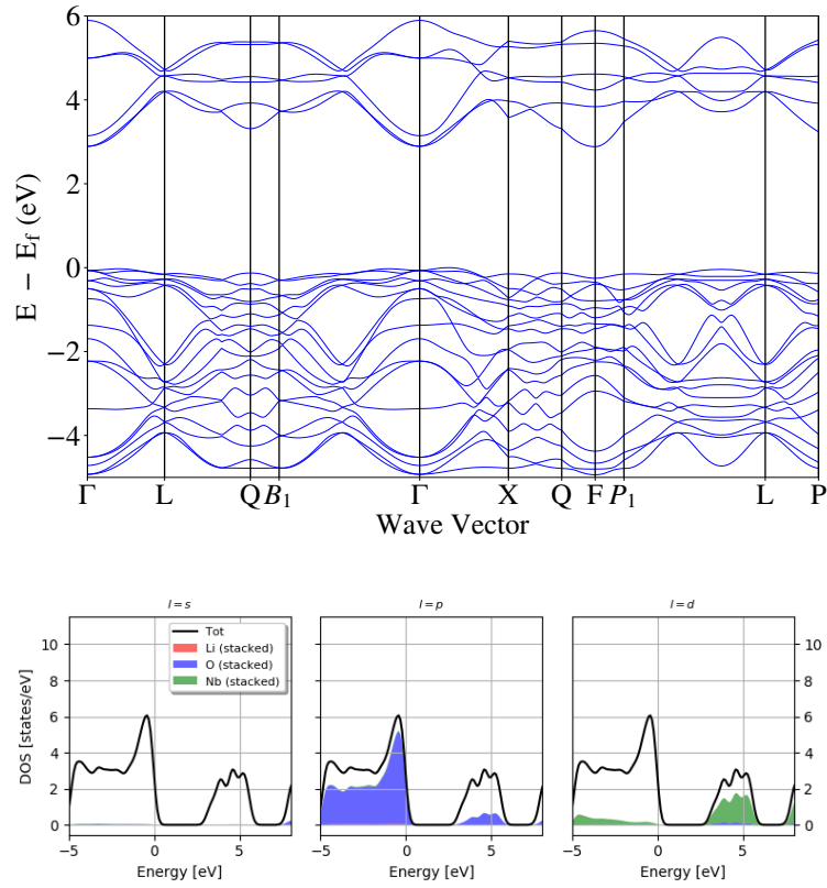
Figure G.3: Electronic structural information of \text{LiNbO}_3 after a second displacement of the atoms from its centrosymmetric positions (Fig. 4.20(b)).
