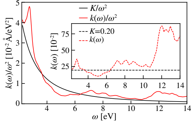
Figure 4.3: Comparison of the frequency-dependent transition probability k(\omega)/\omega^2 and its constant value K/\omega^2 obtained from Eq. (4.10) for a real material ( \text{TiO}_2 , mp-2657). In the inset the comparison is given for k(\omega) and K . All functions are shown in a frequency range [2, \omega_{max}] , with \omega_{max} equal to 14 eV for this material.
