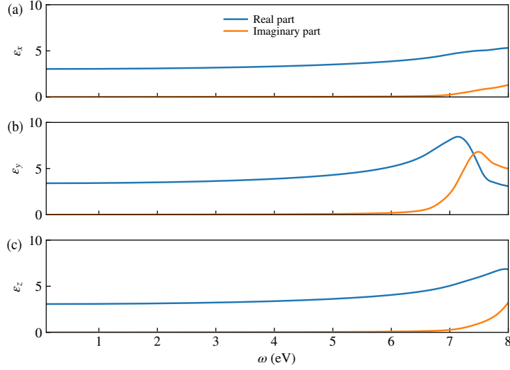
Figure 4.30: Real and imaginary part of the dielectric function of PON as a function of the frequency ((a) x component, (b) y component, (c) z component).
