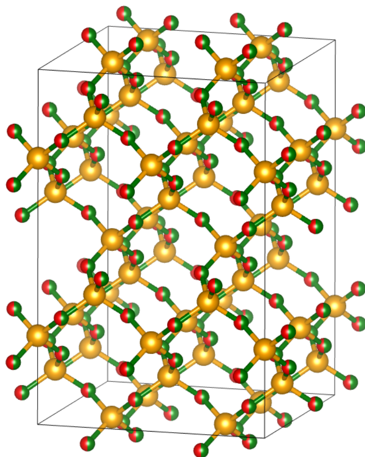
Figure 4.28: Atomic structure of PON, considering a (2 \times 2 \times 2) supercell. The P atoms are colored in yellow, the O atoms are in red, and the N atoms are colored in green.
