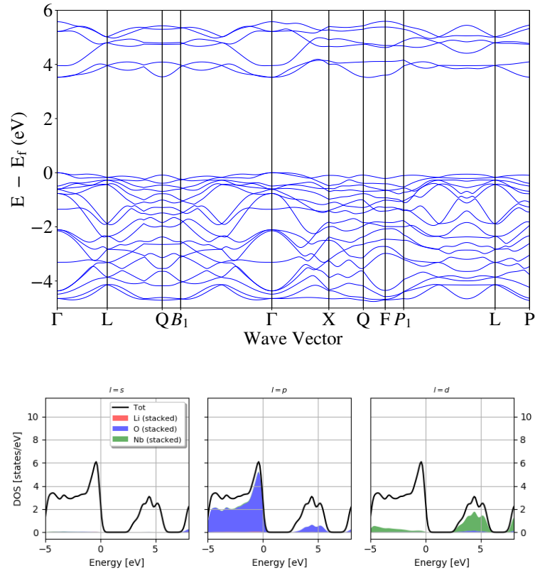
Figure G.5: Electronic structural information of \text{LiNbO}_3 after a fourth displacement of the atoms from its centrosymmetric positions (Fig. 4.20(d)).
