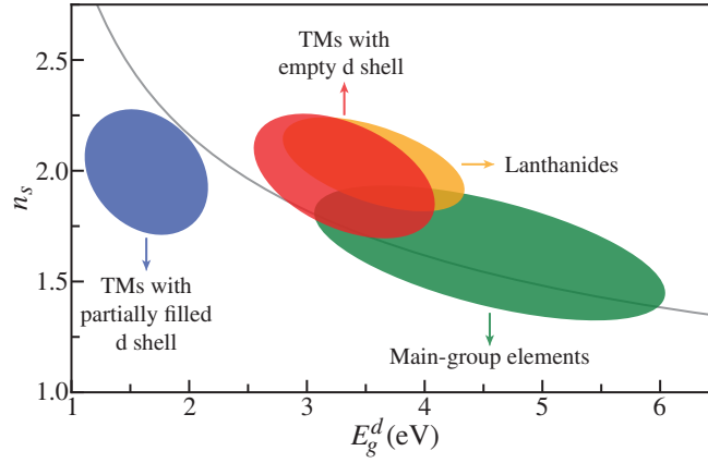
Figure 4.10: Static refractive index n_s as a function of the direct band gap E_g^d for the four classes of materials (first and second groups of TMOs in red, and blue respectively, main-group elements in green, lanthanides in orange) considered in this study. Each class is represented by an ellipse (see text) indicating the main distribution of the materials that belong to this class. The solid line correspond to Eq. (4.18) with \omega_{\text{eff}}=12.10 eV.
