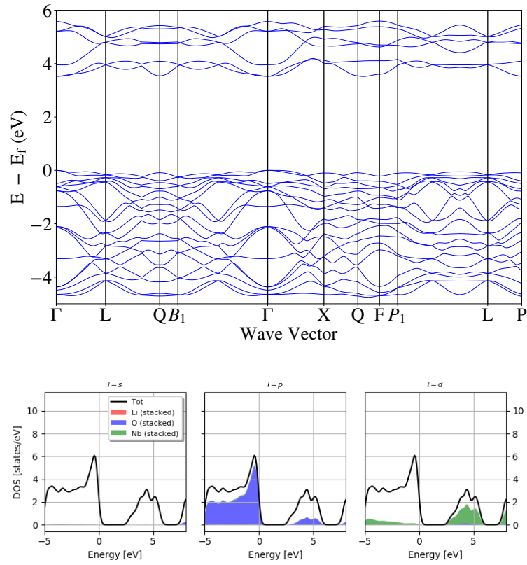
Figure G.6: Electronic structural information of LiNbO 3 in its non-centrosymmetric phase (Fig. 4.19(b)).
