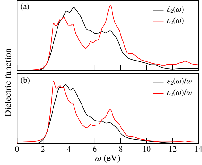
Figure 4.4: Comparison of the imaginary part of (a) the dielectric function \epsilon_2(\omega) and (b) \epsilon_2(\omega)/\omega considering the two methodologies of calculation for a real material (TiO 2 , mp-2657). The red curves are obtained averaging the diagonal components of the DFT imaginary part of the dielectric function (Eq. (4.1)). The black curves are obtained via a renormalization of the j(\omega) (Eq. (4.9)).
