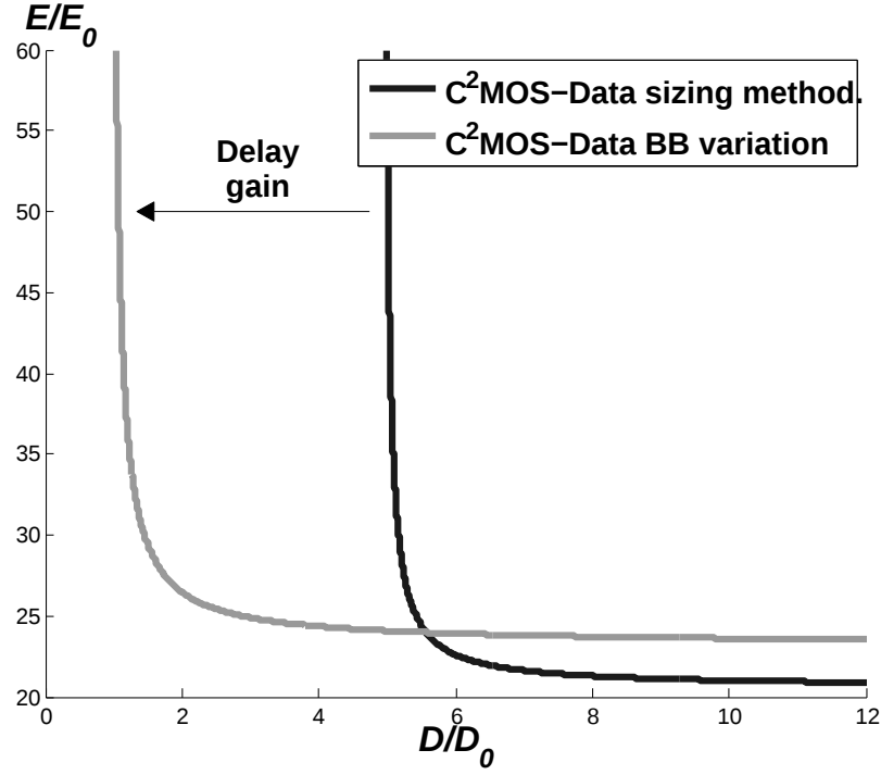
Figure 2.14: EECs of the C 2 MOS-Data architecture extracted from the sizing methodology and from a applied back biasing ( V_{dd} = 0.35\text{V} , driving strength X1, \alpha_{sw} = 0.15 , T_{clk} = 40FO4 , temperature 25^\circ\text{C} ).
