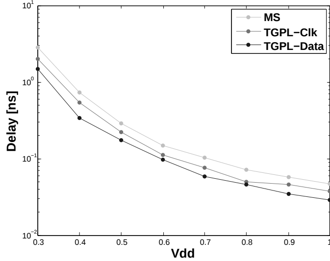
Figure 2.16: Measured delays from 0.3V to 1V in nominal case ( V_{DDS}=G_{NDS}=0V ). Clk-to-Q delay is lower for TGPL-Data than for TGPL-Clk, contrary to the D-to-Q delay ( T^\circ = 80^\circ C ).
