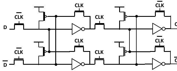
Figure 1.9: Improved MS-based differential structure [34].
