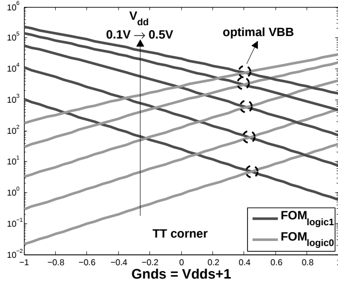
Figure 3.13: For V_{dd} and G_{nds} values evolving in the same way, an optimal point is found near the middle of the diagonal 2 (Fig. 3.11).
