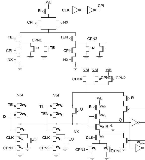
Figure A.4: R-S CPFF architecture.
