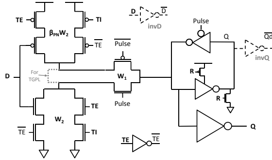
(b) The C 2 MOS-XOR latch with additional inverters for \bar{D} and \bar{Q}_d signals.
