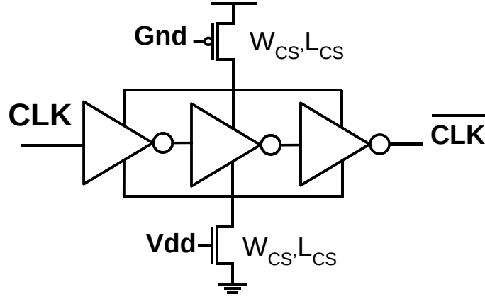
Figure 3.2: Proposed current starved (CS) pulse generator architecture [70].
