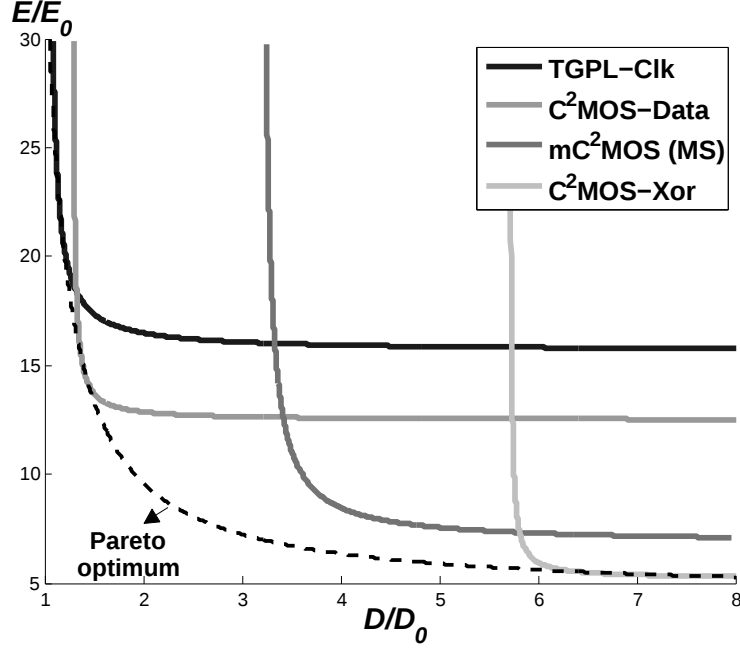
Figure 4.5: EECs for the four interesting architectures at V_{dd} = 1V (driving strength X1, \alpha_{sw} = 0.15 , T_{clk} = 40FO4 , temperature 70^\circ C ). The dashed curve is only there to illustrate the Pareto optimum idea.
