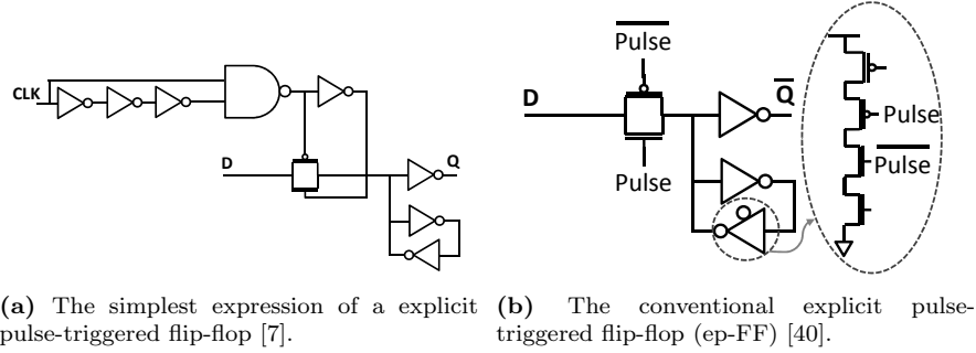
Figure 1.15: The basic structures of explicit pulse-triggered flip-flop.
