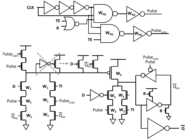
Figure 2.8: Scannable and resettable version of the two-stages single-edge CDFF from figure 1.17d
