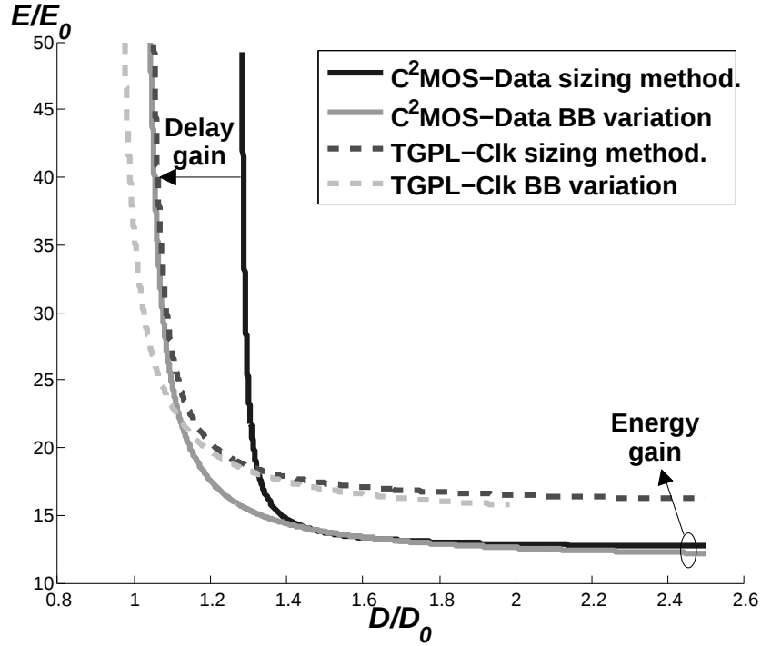
Figure 2.13: EECs of the C 2 MOS-Data and TGPL-Clk architectures extracted from the sizing methodology and from a applied back biasing ( V_{dd} = 1V , v_{dds}/gnds range = \pm 1V , \alpha_{sw} = 0.15 , T_{clk} = 40FO4 , temperature 70^\circ C ). Back biasing technique provides better performances than sizing methodology.
