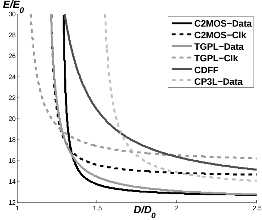
Figure 2.11: EEC: V_{dd} = 1.0V , v_{dds}=gnds=0V , \alpha_{sw} = 0.15 , T_{clk} = 40FO4 , corner TT, temperature 70^{\circ}C .
