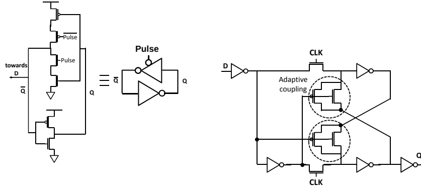
(a) Breaking feedback mechanism in a latch. (b) The adaptive coupling pulsed latch (ACPL) with input data as breaking signal (inspired by [48]).
