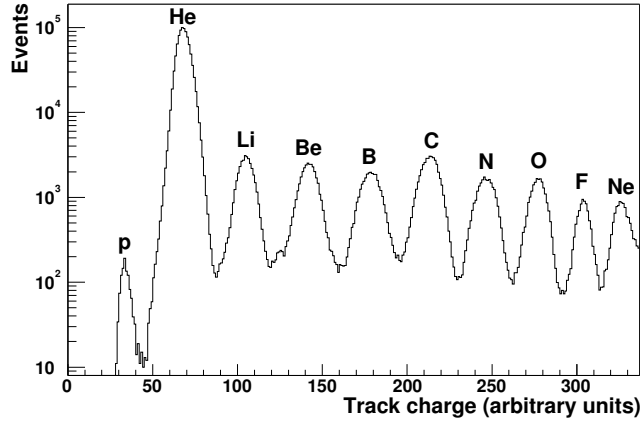
Figure 2. n-side distribution of \sqrt{dE/dx} \sim Z in arbitrary units for a run in the 2002 test. Besides the He peak, up to Z=10 smaller peaks can be easily recognized. Please note the logarithmic scale on the y-axis.
