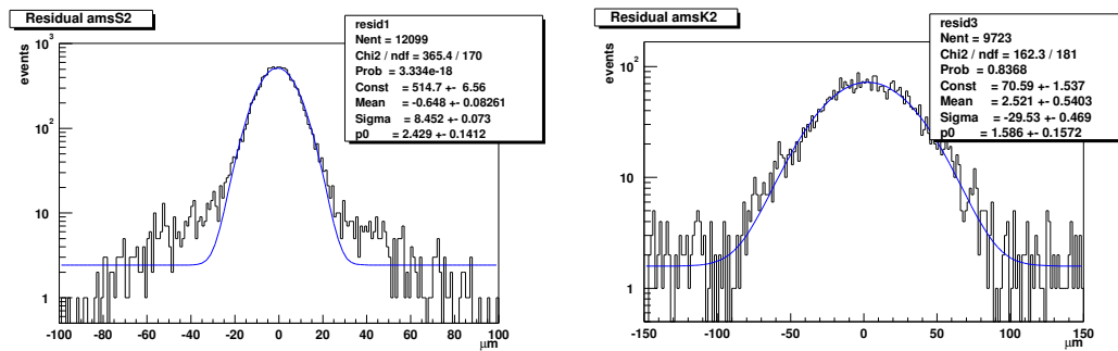
Figure 1. Residua distribution of hits obtained on the prototype ladder in the 2000 test with respect to the position estimated by the beam telescope. Left plot corresponds to p-side and right plot to n-side.
