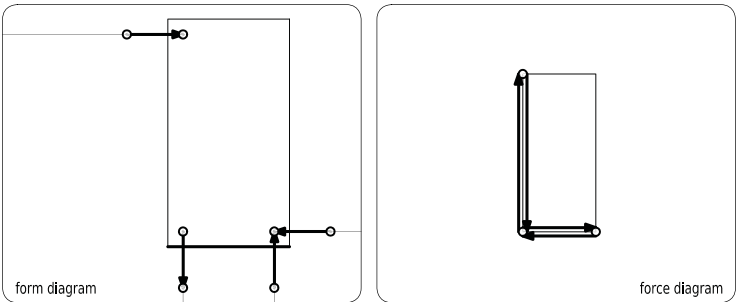
figure 83 application example of a BasicShearPanel object.
