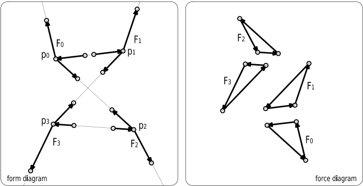
figure 120 these force polygons cannot be joined to form rods.
