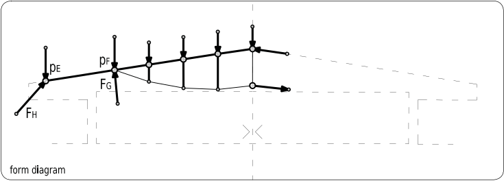
figure 322 reconstruction of Maillart's Chiasso sheds (snapshot 6); the linear domain of p_H , p_I , p_J and p_K are highlighted.
