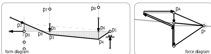
figure 329 bending moment distribution.
