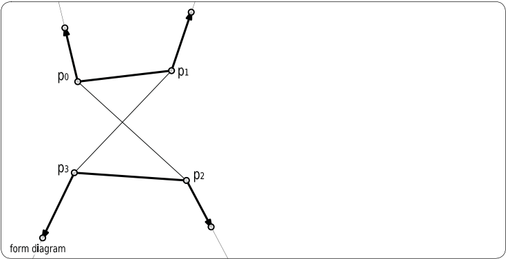
figure 119 a strut-and-tie network that do not satisfy the axiomatic set.
