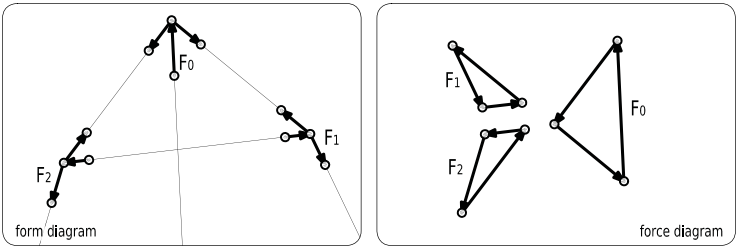
figure 123 these force polygons cannot be joined to form rods.
