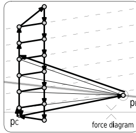
figure 320 reconstruction of Maillart's Chiasso sheds (snapshot 4); the linear domain of p_B is highlighted.
