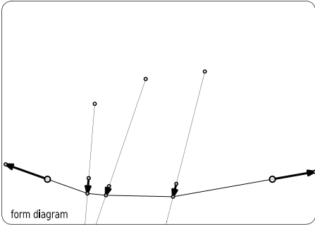
figure 26 a new strut-and-tie network is created to bear the new temporary forces created in figure 25.
