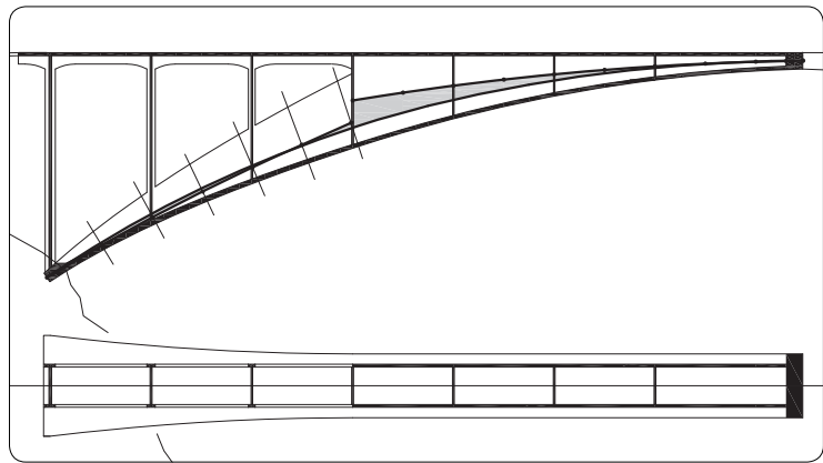
figure 3 description of half of the Salginatobel bridge designed by Robert Maillart; the line of thrust is the continuous curve and the line of centroids consists of two discon- nected curves.
