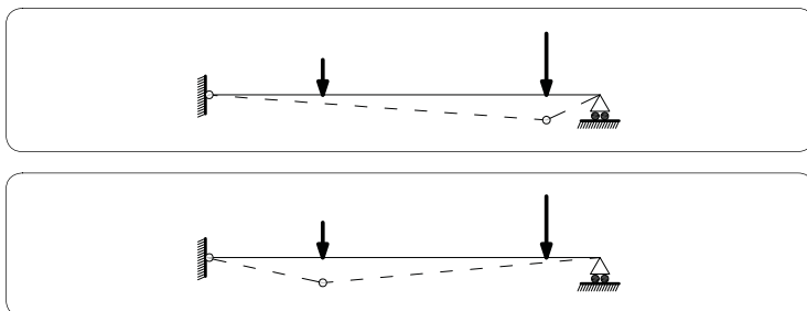
figure 328 two possible collapse mechanisms.
