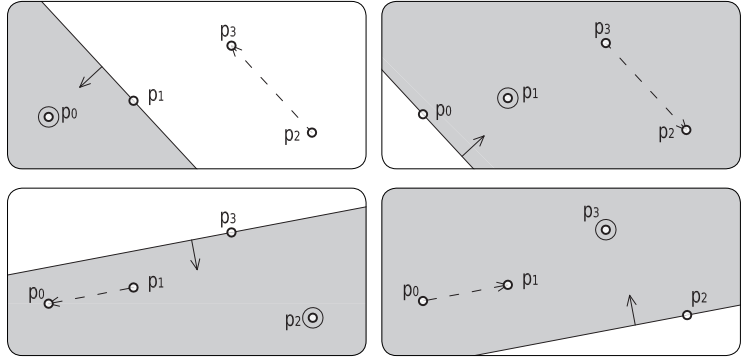
figure 144 four points holding a Laterality [ p_0 p_1 p_2 p_3 ] relationship, each of them belongs to a HalfPlane region.
