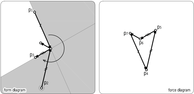
figure 100 in grey, the region in which p_2 must stay in order to ensure a clockwise reading cycle; the force defined by p_2 exerts a push.
