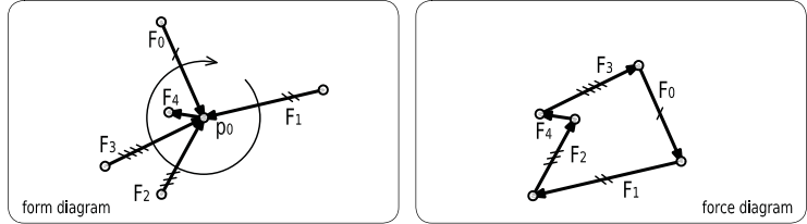
figure 98 five consecutive forces read clockwise.
