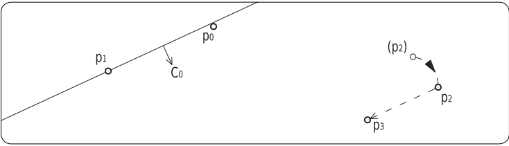
figure 160 move of p_2 , it rotates the half-plane.
