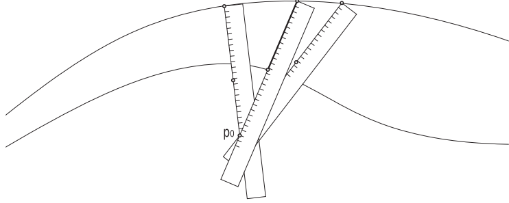
figure 209 a traditional Neusis construction.
