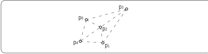
figure 53 axiom T.11, upper dimension.
