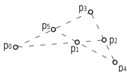
figure 51 axiom T.9, outer Pasch (two examples).
