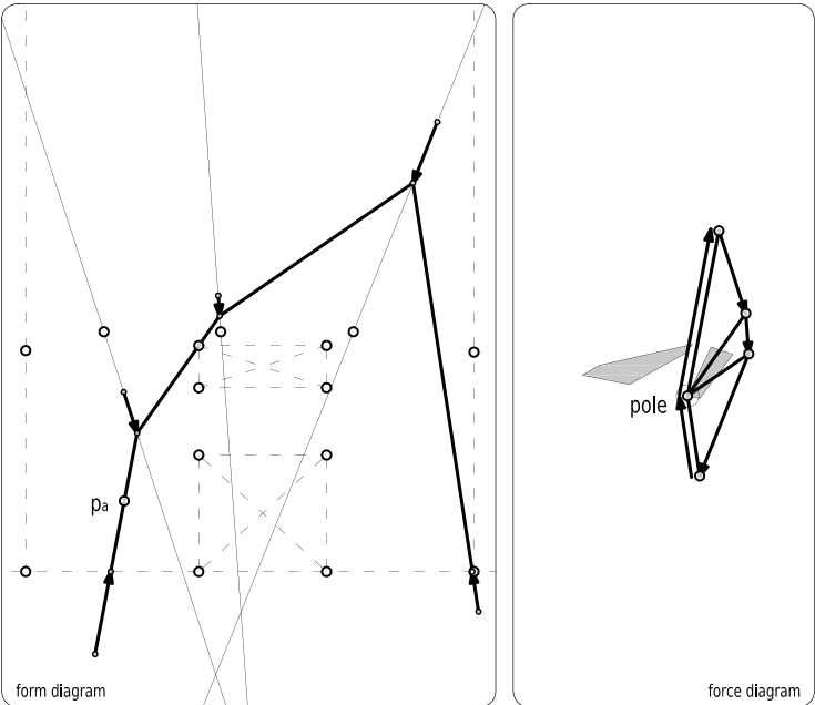
figure 22 reproduction of the construction in figure 20 in which the pole has been moved onto another particular position.
