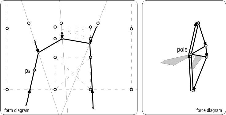
figure 21 reproduction of the construction in figure 20 in which the pole has been moved onto a particular position.
