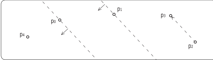
figure 45 five points showing the transitivity of Laterality.
