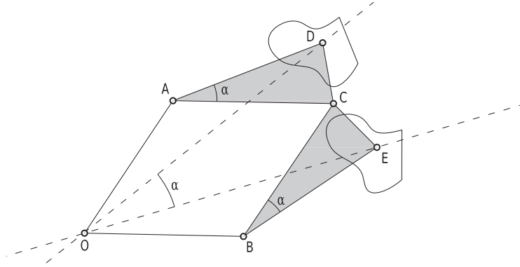
figure 205 mechanism of Sylvester's plagiograph.
