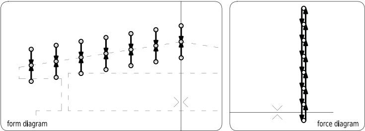
figure 317 reconstruction of Maillart's Chiasso sheds (snapshot 1); initial set of loads.
