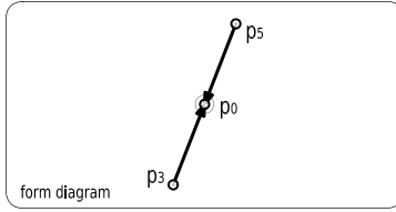
figure 92 first application of Ax.24 upon Ax.23.
