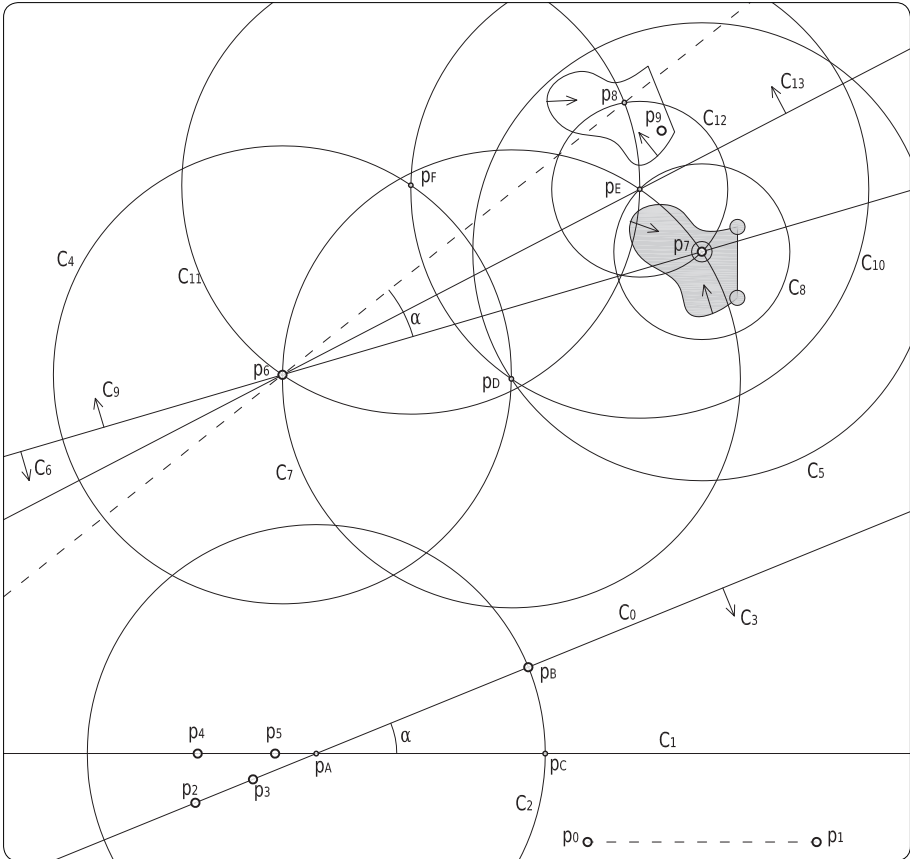
figure 206 construction of p_8 \in \text{Plagiograph } [p_0 p_1, p_2, p_3, p_4, p_5, p_6, p_7] constraint; the domain of p_7 is highlighted.
