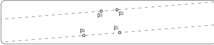
figure 57 four points holding a Parallelism [ p_0 p_1 p_2 p_3 ] relationship.
