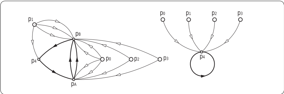
figure 222 construction of p_4 \in \text{Hyperbola } [p_0 p_1 p_2 p_3 p_4] constraint and its graph of dependencies.
