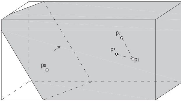
figure 341 mnemonic description of the \text{Laterality}_3\text{D} relationship.
