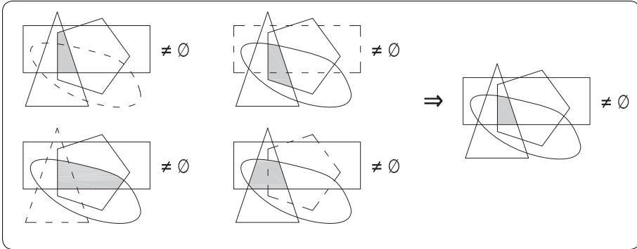
figure 241 basic illustration of Helly's theorem.
