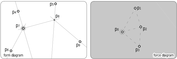
figure 225 prior to permutation; (left) the domain of p_7 is the shaded position; (right) the domain of p_0 is the shaded area.
