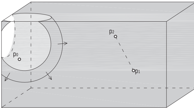
figure 344 representation of a SphereOutside [p_0p_1p_2] fundamental constraint
