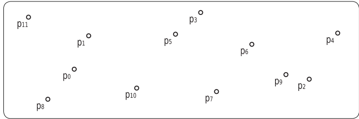
figure 35 a cloud of points.
