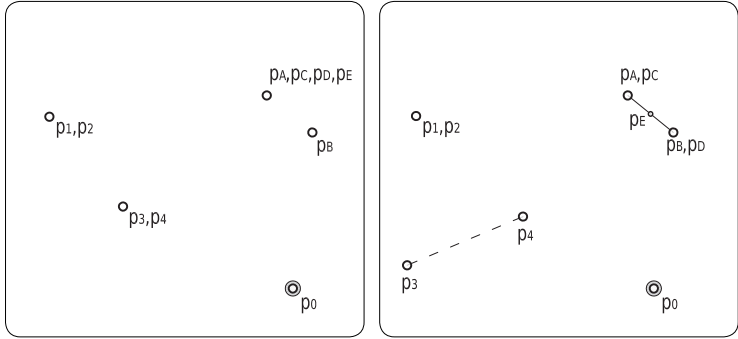
figure 279 the domain of the Disjunctive Condition constraint (left) when Coincidence [p_1 p_2] \vee Coincidence [p_3 p_4] and (right) when Coincidence [p_1 p_2] \vee \neg Coincidence [p_3 p_4] .
