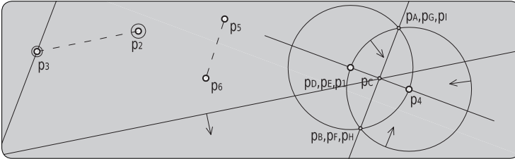
figure 258 the domain of p_2 so that HalfPlane [p_1 p_2 p_3] \cap \text{DiscInside}[p_4 p_5 p_6] is not empty.
