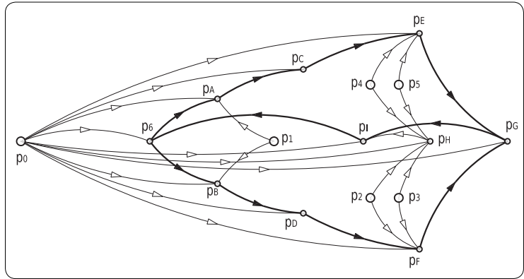
figure 223 construction of p_6 \in \text{Hankinson } [p_0 p_1 p_2 p_3 p_4 p_5 p_6] constraint and its graph of dependencies.
