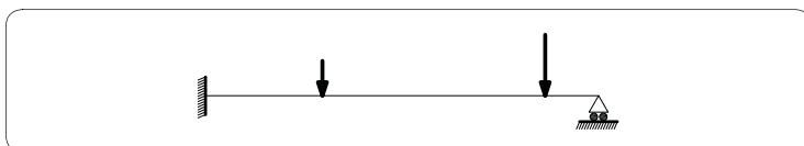
figure 327 initial settings for the clamped beam.
