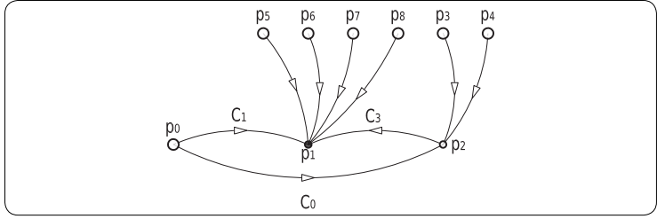
figure 268 directed graph of dependencies after permutation.
