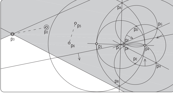
figure 257 the domain of p_2 so that HalfPlane [p_1 p_2 p_3] \cap \text{DiscInside}[p_4 p_5 p_6] is not empty.
