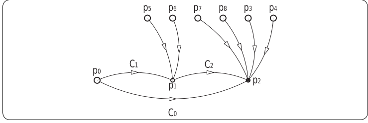
figure 267 directed graph of dependencies prior to permutation.
