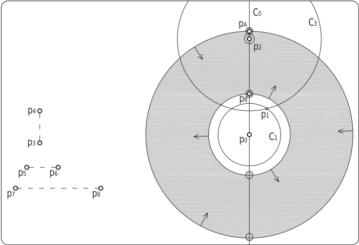
figure 269 the propagation domain of p_2 .
