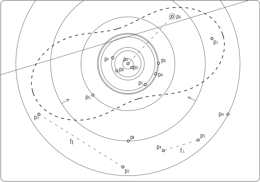
figure 223 construction of p_6 \in \text{Hankinson } [p_0 p_1 p_2 p_3 p_4 p_5 p_6] constraint and its graph of dependencies.
