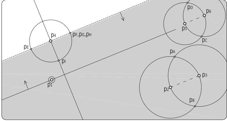
figure 255 the domain of p_1 so that \text{HalfPlane}[p_1 p_2 p_3] \cap \text{HalfPlane}[p_4 p_5 p_6] is not empty.
