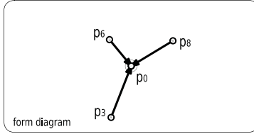
figure 93 second application of Ax.24 upon Ax.23.
