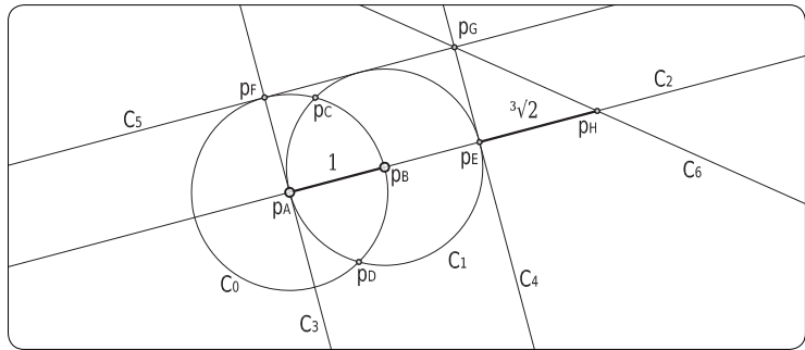
figure 215 construction of a CubicRootOfTwo Compass[ p_3 ] constraint.
