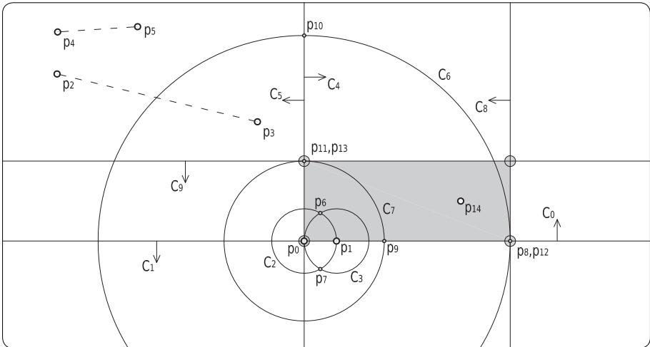
figure 283 a rectangle whose longest side is always horizontal.
