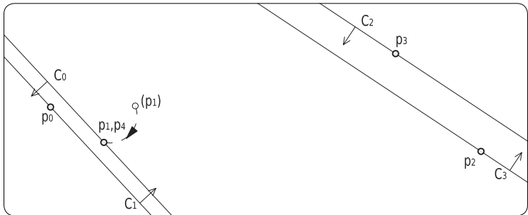
figure 151 final move of p_1 .
