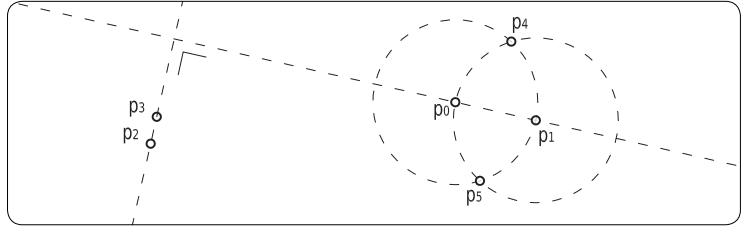
figure 59 four points holding a Orthogonality [ p_0 p_1 p_2 p_3 ] relationship.
