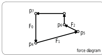
figure 284 the domain that p_2 must hold in order to guarantee Ax.27.
