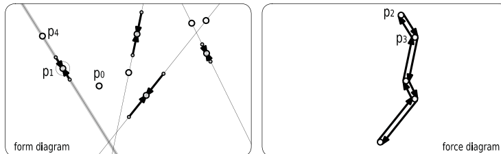
figure 310 initial situation before the execution of the CreateCatenary procedure; the domain of p_1 is highlighted.
