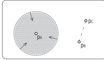
figure 141 a DiscOutside [p_A p_B p_C] region (left) and its inverse (right).
