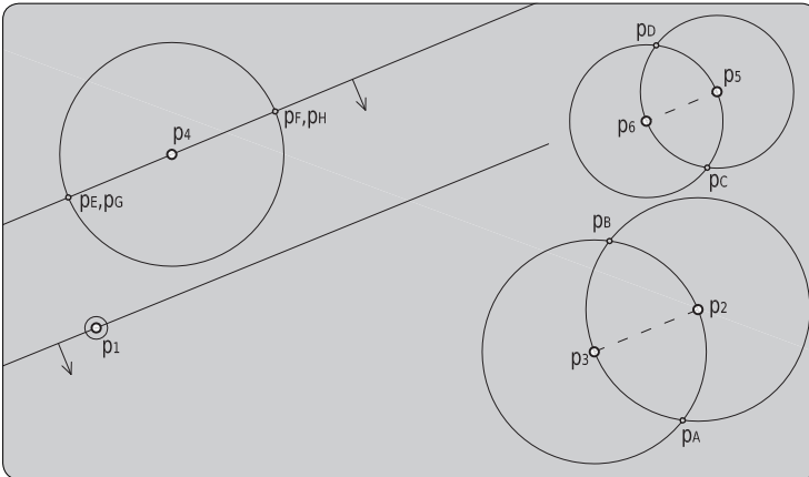
figure 249 the domain of p_1 so that HalfPlane [p_1 p_2 p_3] \cap HalfPlane [p_4 p_5 p_6] is not empty.
