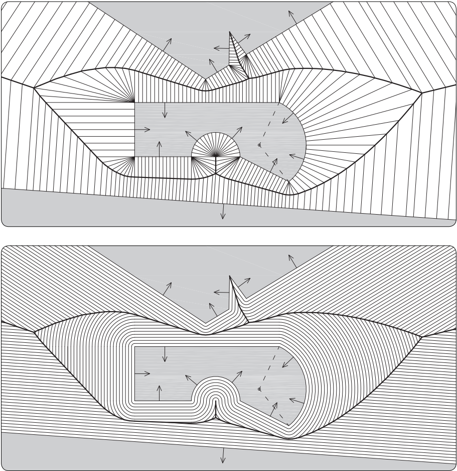
figure 163 if the region (grey area) is not empty, every position has a closest point.
