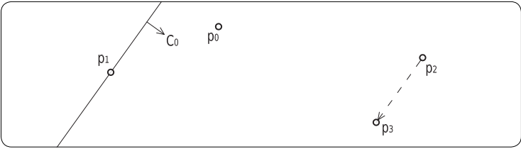
figure 159 a point p_0 constrained on a half-plane.
