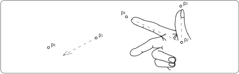
figure 341 mnemonic description of the \text{Laterality}_3\text{D} relationship.
