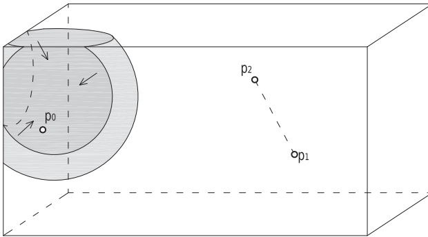
figure 343 representation of a SphereInside [p_0p_1p_2] fundamental constraint.
