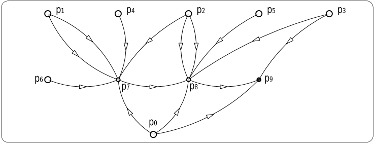
figure 226 directed graph of dependencies before permuta- tion.
