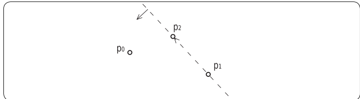
figure 44 three points holding the \text{Laterality}[p_0 p_1 p_1 p_2] and \text{Laterality}[p_0 p_2 p_1 p_2] relationships.
