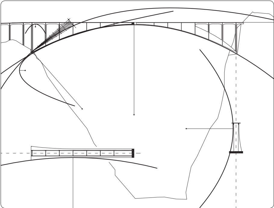
figure 4 reconstruction of some parabolas that Robert Maillart drew on the first working-drawings for the Salginatobel bridge; the bundle of lines depict the construction process of a parabola from two crossing-points and the orientation of a directrix.
