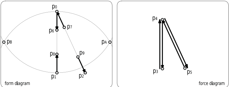
figure 82 the geometric pattern of the BasicShearPanel relationship.
