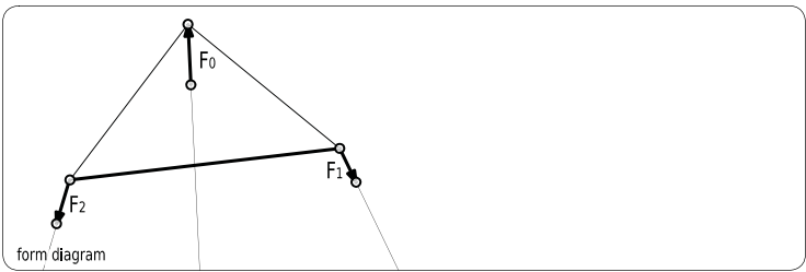
figure 122 a strut-and-tie network that do not satisfy the axiomatic set.
