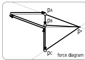
figure 330 bending moment distribution.
