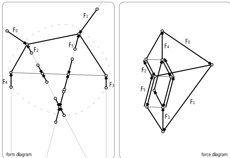
figure 137 intermediate hull containing the entire strut-and- tie network from figure 135.
