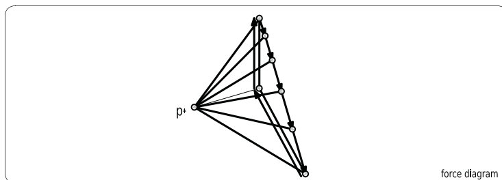
figure 8 Force diagram associated with the strut-and-tie network shown in figure 6.
