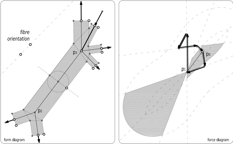
figure 339 a rectilinear stress field: dragging p_0 will cause the rectilinear stress field to be rotated around p_3 or to switch from traction to compression; as long as p_0 remains within its graphical domain of solution (the shaded area in the force diagram), the strength of this stress field is ensured to be below the plastic limit of the wood; the asymmetrical curvy shape of this domain of solution is due to the anisotropic nature of wood.
