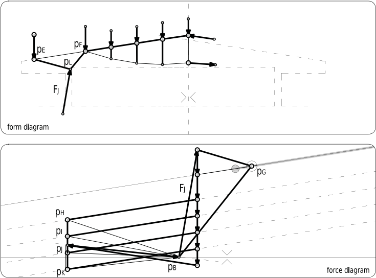
figure 323 reconstruction of Maillart's Chiasso sheds (snapshot 7); the linear domain of p_G is highlighted.
