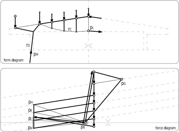
figure 324 reconstruction of Maillart's Chiasso sheds (snapshot 8); the linear domain of p_B is highlighted.
