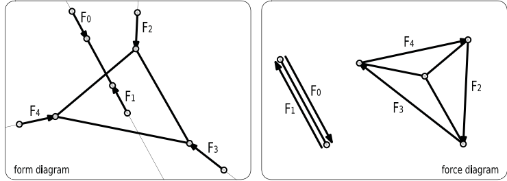
figure 130 two strut-and-tie networks with an intersection of rods.
