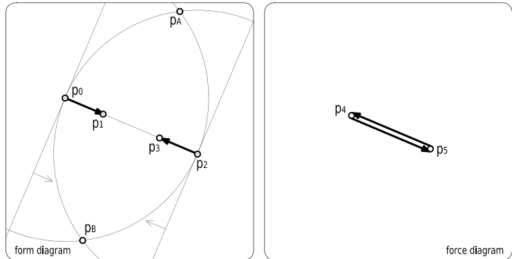
figure 75 two forces fulfilling all the prerequisite conditions in a way that they can be considered as a rod.
