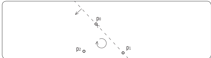
figure 62 three points holding a ClockWiseness [ p_0 p_1 p_2 ] relationship.
