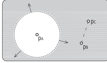
figure 140 a DiscInside [p_A p_B p_C] region (left) and its inverse (right).
