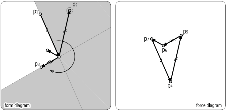
figure 99 in grey, the region in which p_2 must stay in order to ensure a clockwise reading cycle; the force defined by p_2 exerts a pull.
