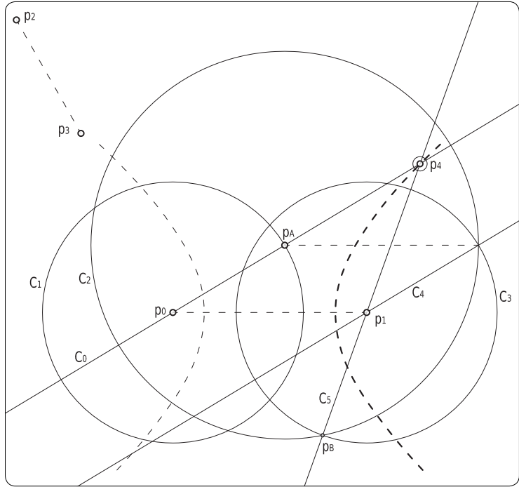
figure 222 construction of p_4 \in \text{Hyperbola } [p_0 p_1 p_2 p_3 p_4] constraint and its graph of dependencies.
