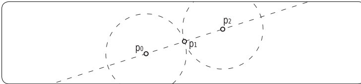
figure 58 three points holding a MidPoint[ p_0 p_1 p_2 ] relationship.
