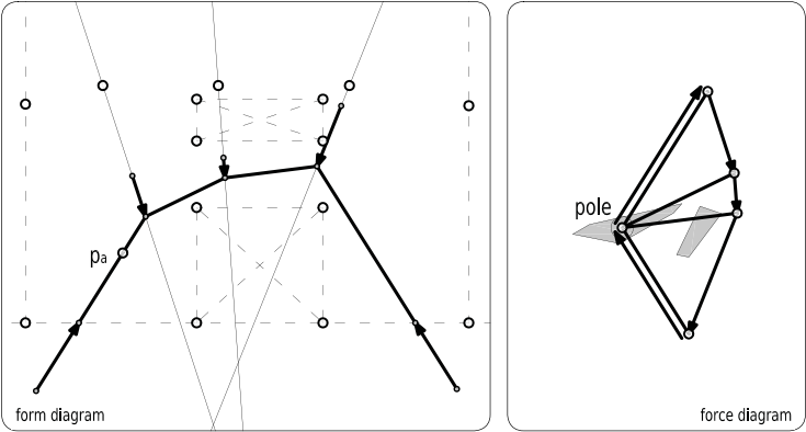
figure 20 the grey area in the force diagram shows the possible positions of the pole if the funicular polyline has to stay outside the shapes drawn in the form diagram.
