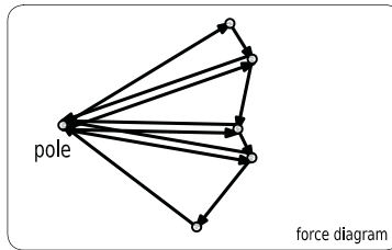
figure 311 creation of the pole and resolution of forces.
