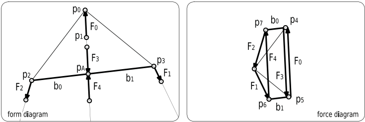
figure 124 adding a point at the intersection of the rod with the half-line of force makes the network compatible with the axiomatic set.
