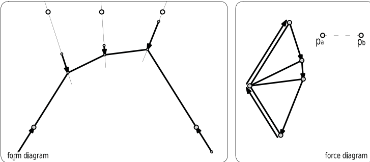
figure 24 initial situation: forces are supported by a funicular polyline but the magnitude of the compression rods are too high.
