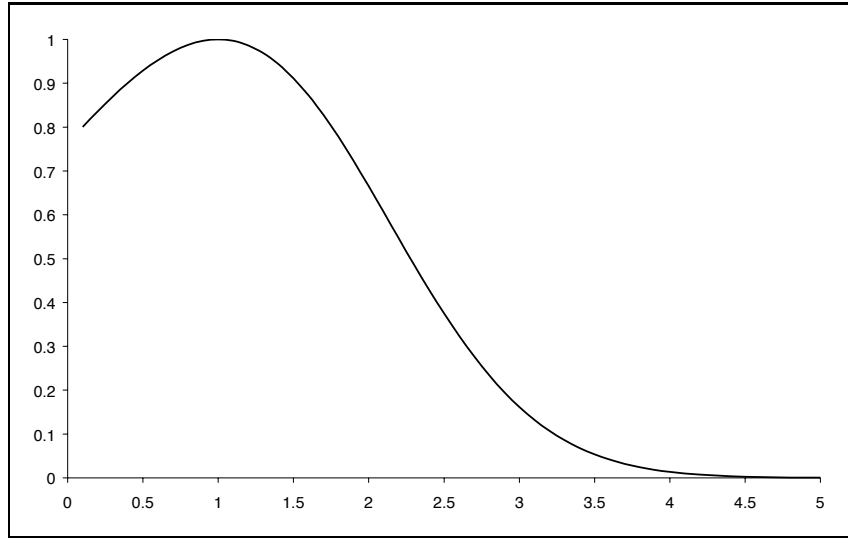
Figure 5: The correlation coefficient of the comonotonic random couple (X_1, X_2) .
