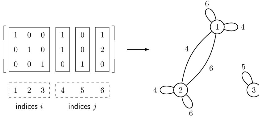
Fig. 1. Example of matrix \mathbf{A} and the associated graph G .
