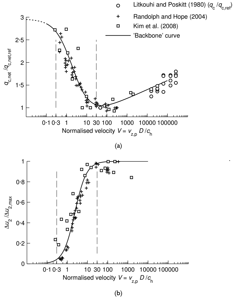
Figure 2.6 (a) Cone resistance and (b) Excess pore pressure behind the shoulder versus normalised penetration velocity V .
