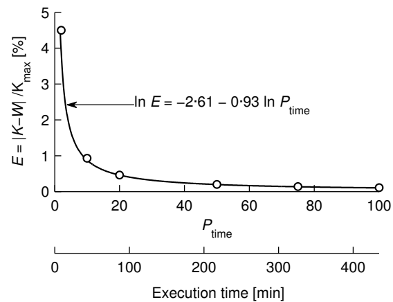
Figure E.7 Error between kinetic energy and work versus the critical time increment parameter P_{\text{time}} .
