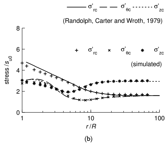
Figure E.11 Distribution of effective stresses (a) after cavity expansion and (b) subsequent consolidation.
