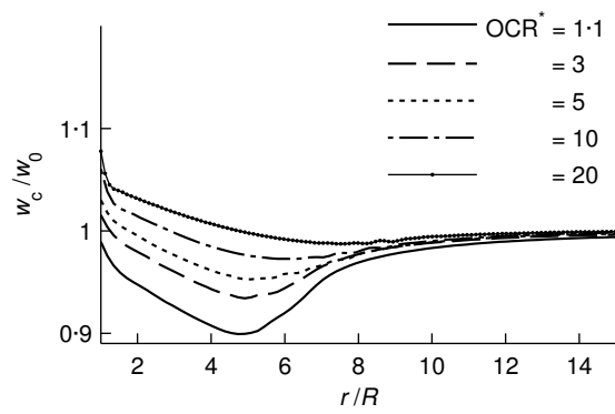
Figure F.14 Distribution of water content after equalisation.
