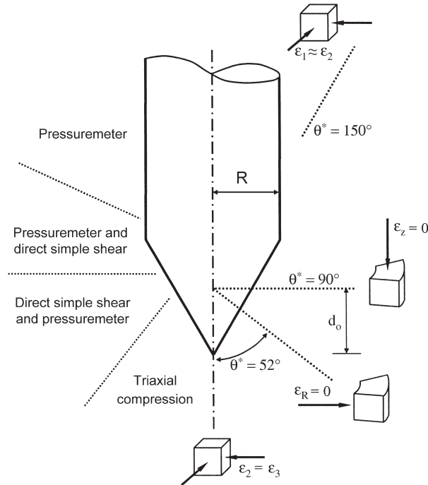
Figure 3.9 Presumed failure modes around an advancing cone, on the left by Keaveny and Mitchell (1986) and on the right by Baligh (1984), both cited by Su (2010).
