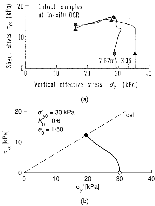
Figure 7.5 Simple shear at in situ state; (a) experiment (Lehane, 1992) and (b) simulation.
