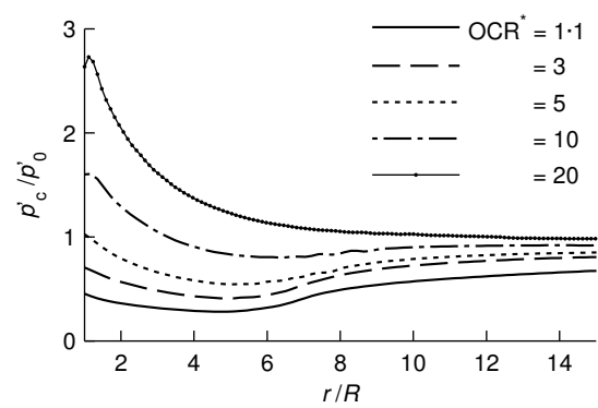
Figure F.12 Distribution of mean effective stress after equalisation.
