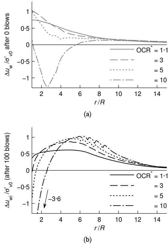
Figure 6.3 Distribution of pore pressure (a) after the Strain Path Method and (b) at the end of installation (after 100 blows of the Disk Shearing Model).
