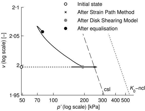
Figure F.10 Stress path at the pile wall in the compression plane for OCR^* = 10 ( OCR = 21.1 ).
