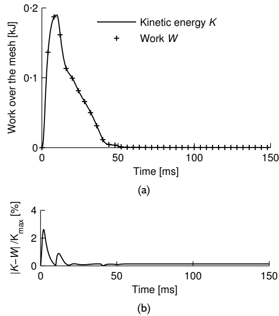
Figure E.6 (a) Work and kinetic energy over the entire domain during a blow for P_{\text{time}} = 50 and (b) Error between these two quantities versus time.
