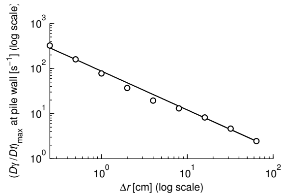
Figure E.10 Maximum shear strain rate \dot{\gamma}_{max} at pile wall for various internodal distances \Delta r , for P_{time} = 50 .
