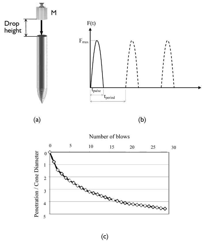
Figure 3.7 Simulation of a dynamic penetration test in an elastoplastic Mohr-Coulomb soil model using the Material Point Method: (a) Hammer and cone geometry, (b) Imposed force at cone head, and (c) Cone penetration ratio versus blow count (Jassim et al., 2013).
