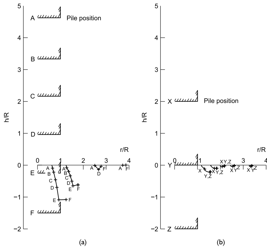
Figure 2.5 Soil trajectories during laboratory pile jacking in (a) spetstone kaolin clay and (b) transparent soil (data respectively from Randolph, Steenfelt and Wroth, 1979 and Lehane and Gill, 2004).
