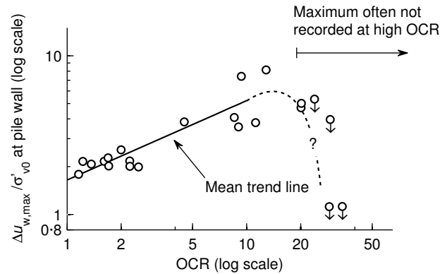
Figure 2.13 Maximum pore pressure recorded at the pile wall during equalisation versus apparent overconsolidation ratio (data compiled by Lehane, 1992).
