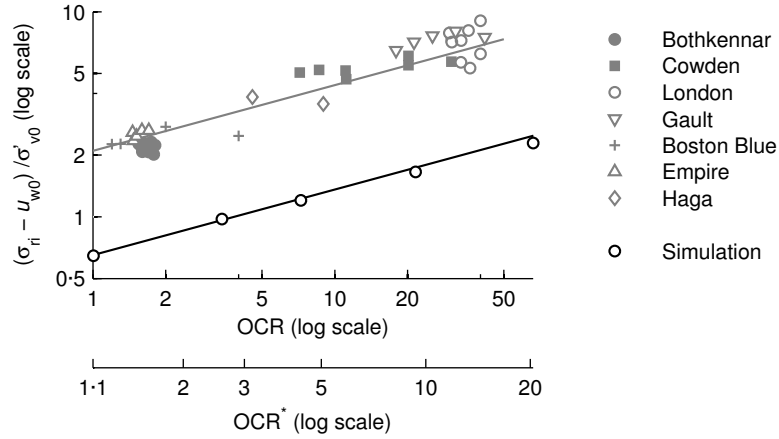
Figure 6.4 Normalised radial total stress after installation versus overconsolidation ratio (hypoplastic OCR^* and conventional OCR ): experiments (reproduced from Fig. 2.10, p. 29; data compiled by Chow, 1996) and simulation.
