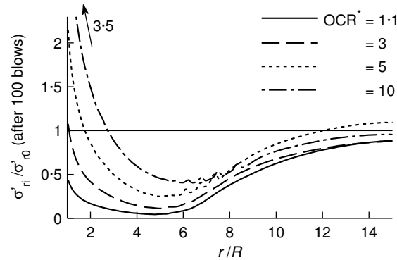
Figure 6.5 Distribution of radial effective stress after installation.
