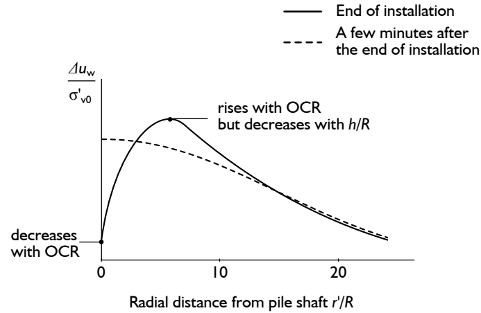
Figure 8.1 Tentative radial distribution of excess pore pressure ratio far behind the pile toe ( h/R > 20 ) immediately and a few minutes after installation.
