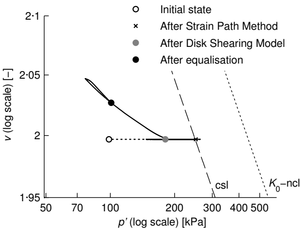
Figure F.9 Stress path at the pile wall in the compression plane for OCR^* = 5 ( OCR = 7.1 ).
