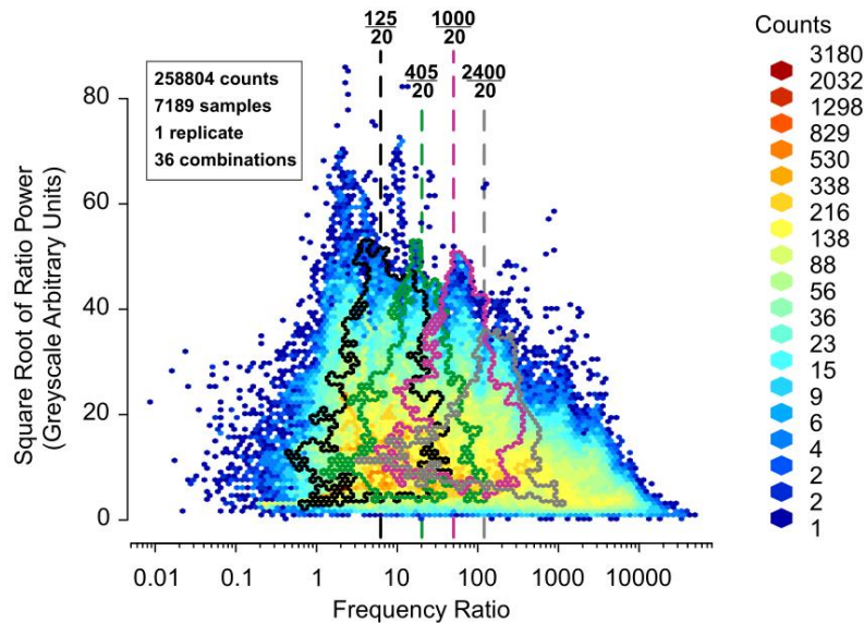
1160 Figure 21: Ratio population for all pairs of components of the decomposition of the greyscale signal of ODP 926. The dotted lines stand for the expected frequency ratios. The black, green, purple and grey contours delineate the ratios of GSC3 with, respectively, GSC 5 to 8. [NOTE TO REVIEWERS: colour online only; 1.5 column fitting image]
