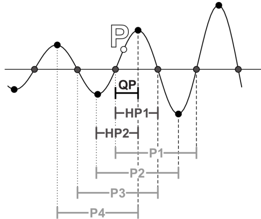
Figure 5: Illustration of the frequency computation by the generalised zero-crossing method. For each point P, the frequency can be computed by making a weighted average of the quarter of the cycle period (QP), two half periods (HP1 and HP2), and four full periods (P1 to P4) that are defined by the extrema and the zero-crossings. [NOTE TO REVIEWERS: 1 column fitting image]
