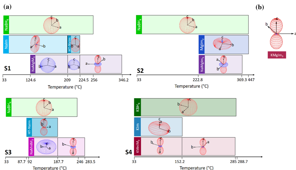
Figure 7 Thermal indicatrices of phases present in samples a S1-S4, b \text{KMgIm}_3 .
