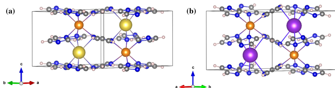
Figure 5 Crystal structure of a NaMnIm 3 and b KMnIm 3 . Manganese atoms are shown as orange balls, sodium as yellow, potassium is given in purple, carbon is grey while nitrogen is shown in blue colour.
