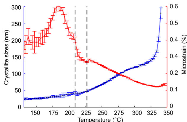
Figure 11 Temperature dependence of the crystallite size (blue) and the microstrain (red) for NaMgIm 3 phase in S1. Vertical dashed lines located at temperatures 209 °C and 227 °C indicate temperature regions with different thermal expansion behaviour.
