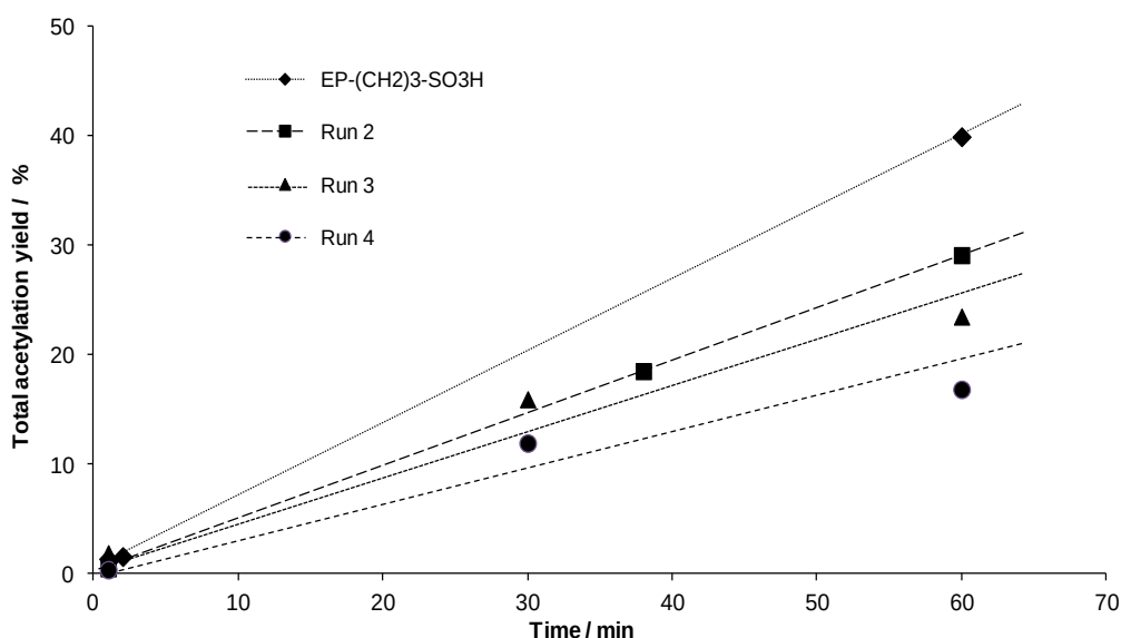
Figure 6. Recyclability experiments for \text{EP}-(\text{CH}_2)_3\text{SO}_3\text{H} with several runs during the first hour of the reaction. The lines are intended as visual aids only.
