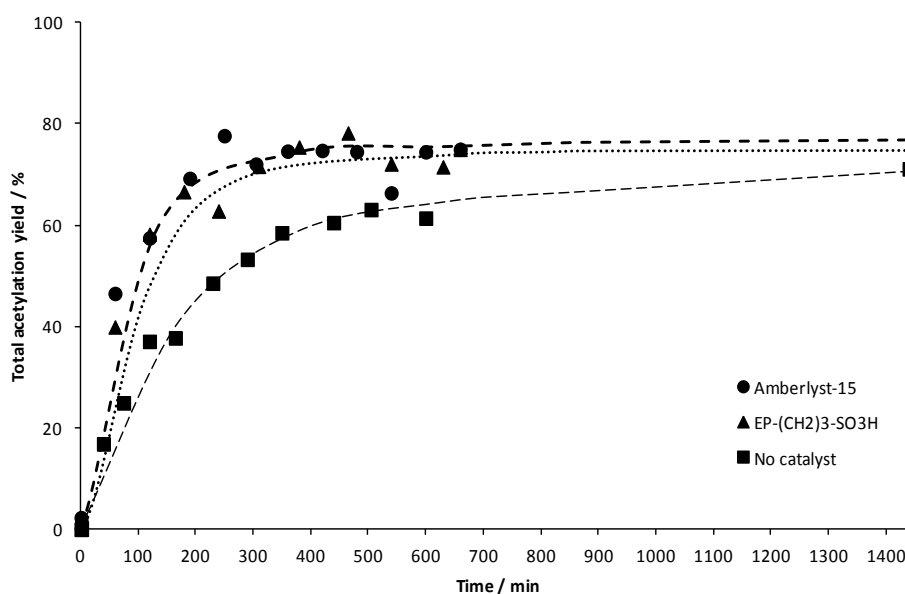
Figure 5. The total acetylation yield for the catalytic reaction with \text{EP}-(\text{CH}_2)_3-\text{SO}_3\text{H} and Amberlyst-15. Also the blank reaction is represented for clarity. A catalyst loading of 0.25 g per 40 mL of glycerol was used. The lines are intended as visual aids only.
