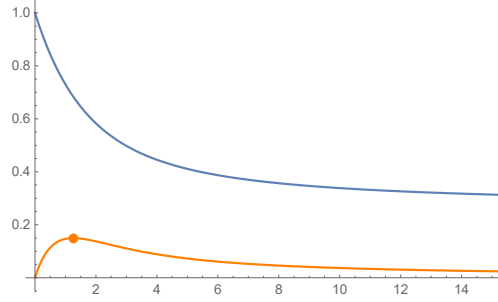
Figure 2: The coefficients s \mapsto b_1(s) (blue) and s \mapsto b_{(1,1)}(s, s) (orange) for \rho = 0.6b^{-\frac{1}{2b}} and b = \frac{13}{10} . The orange dot has coordinates (s_*, b_{(1,1)}(s_*, s_*)) .
