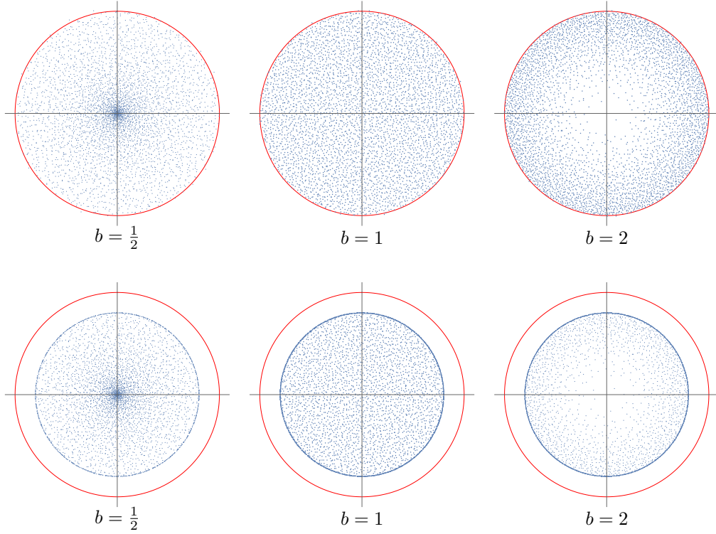
Figure 1: Illustration of the point processes corresponding to (1.7) (first row) and (1.9) (second row) with n = 4096 , \rho = \frac{4}{5}b^{-\frac{1}{2b}} , \alpha = 0 and the indicated values of b . In each plot, the red circle is \{z \in \mathbb{C} : |z| = b^{-\frac{1}{2b}}\} . A narrow interface about the hard wall |z| = \rho , of width roughly 1/n , accommodates the roughly c_\rho n particles swept out from the forbidden region. The semi-hard regime of width roughly 1/\sqrt{n} is transitional between the hard edge and the bulk.
