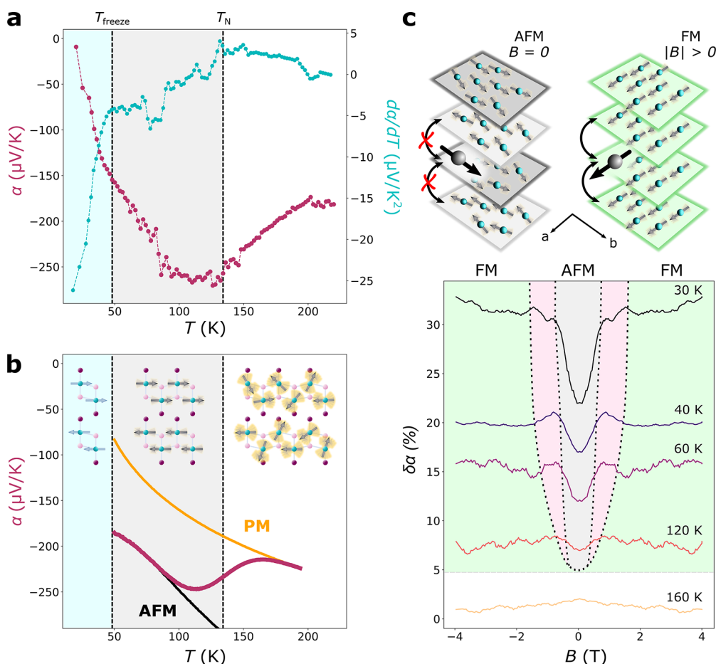
Figure 3. Magnetic field and temperature dependence of the Seebeck coefficient of CrSBr. a) Variation of the Seebeck coefficient (purple curve) and its first derivative (cyan curve) at B = 0 as a function of temperature. The temperatures T_N and T_{\text{freeze}} separate the graph in three areas, colored respectively in white, gray and light blue. b) First-principles Seebeck coefficient as a function of T , for a representative (n-type) doping level, calculated in the AFM (black curve), PM (orange curve), and interpolated magnetic states (purple curve). c) Magneto-Seebeck coefficient as a function of temperature. Each curve is offset by 5% for clarity, and averaged as \frac{\delta\alpha(B) + \delta\alpha(-B)}{2} in order to remove any parasitic effect due to drift in the measurement. The black dotted guidelines delimit the transition region (depicted in pink) in which the spins are canting from AFM (gray area) to FM (green area) ordering and the Seebeck coefficient reaches its maximum. In particular, the external black dotted line between the transition region and the FM state represents the saturation magnetic field H_s (see Supporting Information section S9). The field-dependent spin reorientation and interlayer tunneling is illustrated in the top part of the image. The orientation of the crystallographic axes is also reported. An electron residing on one of the layers (dark gray sphere) can tunnel (indicated by the black curved arrows) or not (indicated by the black curved arrows with red X) depending on its spin orientation.
