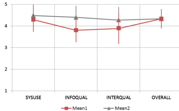
Fig. 8. CSUQ stock chart - Mean1 (resp. 2) refers to mean scores of prototype1 (resp. 2)
