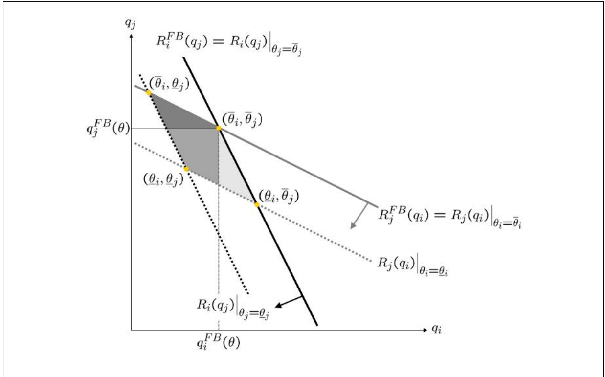
Figure 2: Best-responses and the set of quality levels in the PDP equilibrium.
