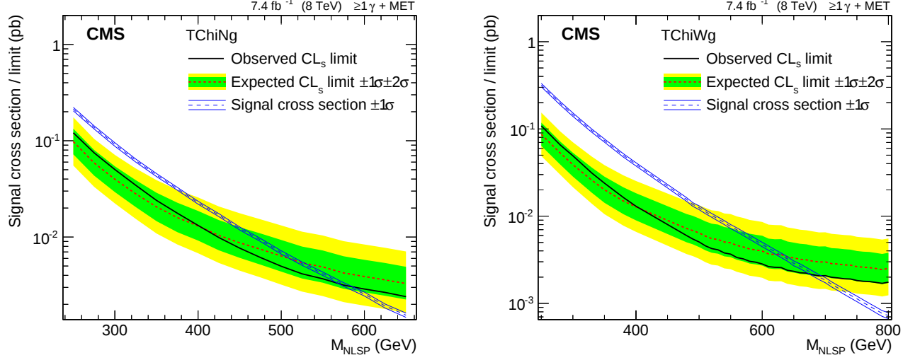
Figure 3: Exclusion limits at 95% CL for the TChiNg (left) and TChiWg (right) scenario. In the TChiNg scenario NLSP masses below 570 GeV are excluded, in the TChiWg scenario NLSP masses below 680 GeV are excluded.
