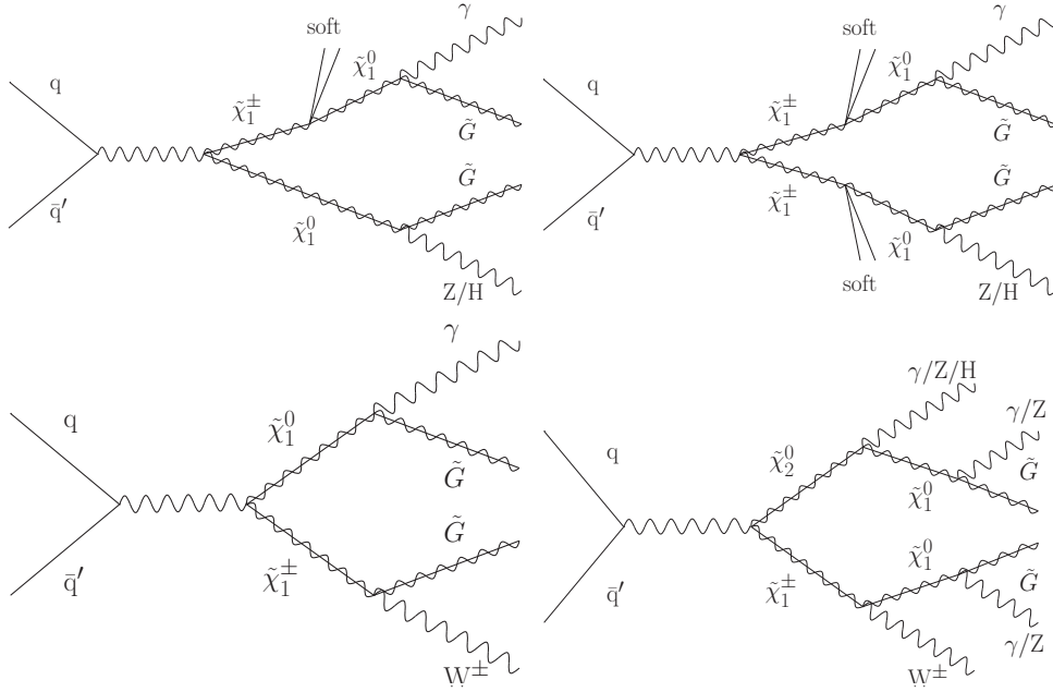
Figure 1: Scenarios for the production and decay of charginos and neutralinos considered in this analysis. In the TChiNg scenario (top row), the charginos are only slightly heavier than the neutralinos, leading to chargino to neutralino decays accompanied by soft radiation. One neutralino decays to a photon and a gravitino, while the other decays into a Z or an H boson and a gravitino with equal probability. In the TChiWg scenario (bottom left), the gauginos are mass-degenerate and the \tilde{\chi}_1^0 decays are as shown. Within GGM models, the \tilde{\chi}_1^0 \rightarrow \gamma\tilde{G} to \tilde{\chi}_1^0 \rightarrow Z\tilde{G} branching fraction depends on the neutralino mass. The dominant process for electroweak GGM production is shown in bottom right. A small amount of hadronic energy and at least one photon and E_T^{\text{miss}} are common features of all scenarios.
