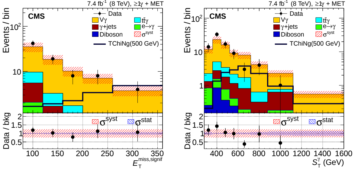
Figure 2: The E_T^{\text{miss, signif}} (left) and S_T^\gamma (right) variables are shown in the signal selection and used to define four search regions with E_T^{\text{miss, signif}} = 200 and S_T^\gamma = 600 GeV partitions. A benchmark TChiNg signal point with an NLSP mass of 500 GeV is shown for comparison.
