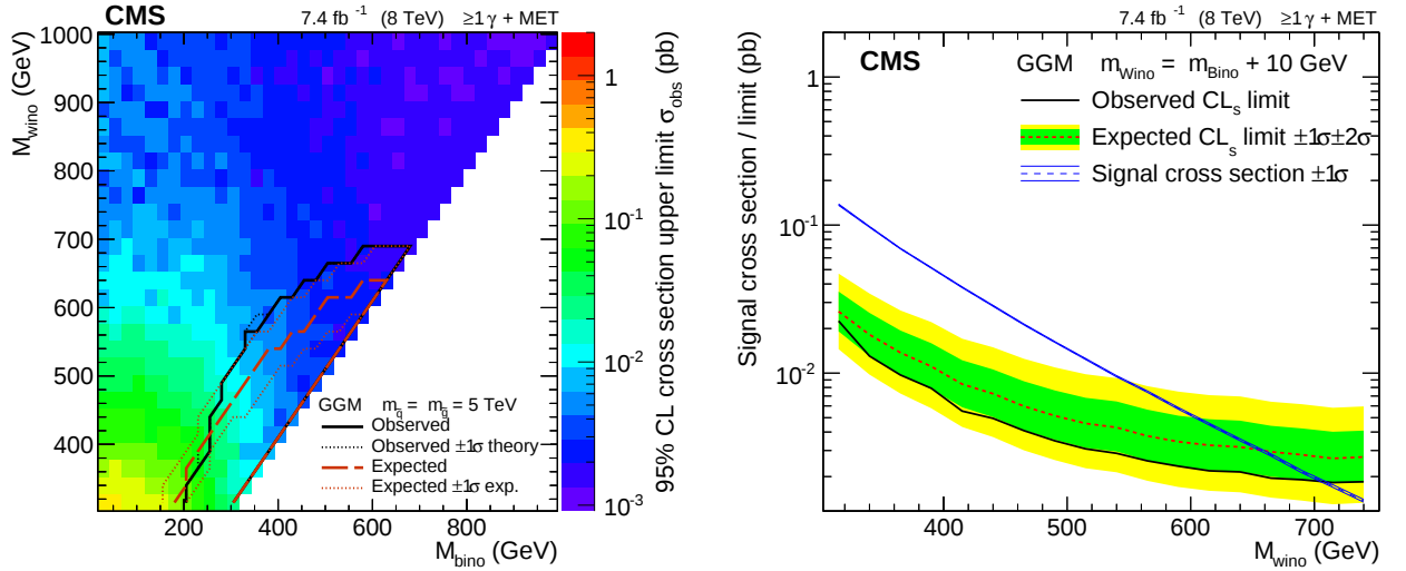
Figure 4: Observed upper cross section CL_s limit at the 95% CL for the GGM signal points in the M_{\text{wino}}-M_{\text{bino}} plane (left). Also shown are the 95% CL expected and observed exclusion contours. The GGM signal points near the diagonal, e.g. for M_{\text{wino}} = M_{\text{bino}} + 10 GeV up to a wino mass of M_{\text{wino}} = 710 GeV are excluded (right).
