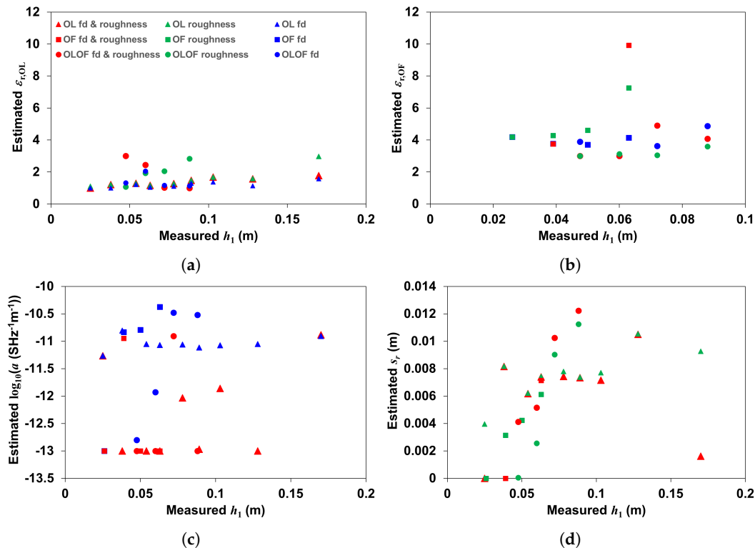
Figure 8. Variations of the estimates of the relative dielectric permittivity (a) of OL litter ( \varepsilon_{r,OL} ) and (b) of OF litter ( \varepsilon_{r,OF} ), (c) of the rate of variation of litter electrical conductivity with frequency ( \log_{10}(a) ) and (d) of the standard deviation of litter surface height ( s_r ) as a function of measured litter thickness of the controlled experiment. The OL, OF and OL-OF litter configurations (see Figure 1) are considered for, respectively, the OL, OF and OLOF litter types. Results are presented for the model considering only frequency dependence of litter effective electrical conductivity reported by André et al. [33] (blue markers), for the model accounting for both surface roughness and frequency dependence of litter effective electrical conductivity (red markers) and for the model considering surface roughness only (green markers). Marker types specify litter configurations.
