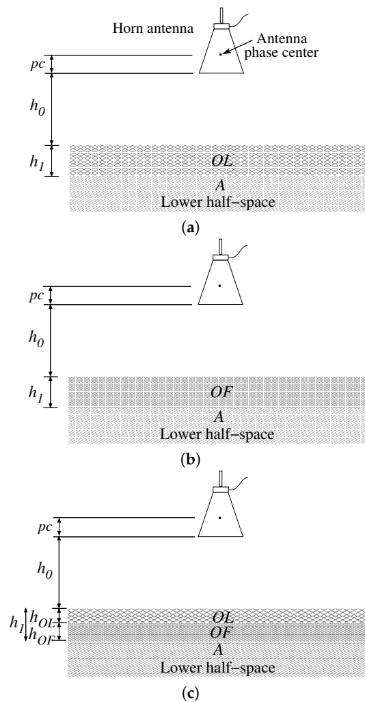
Figure 1. Schemes of the experimental setup for (a) the single recently fallen (OL) layer, (b) the single fragmented (OF) layer and (c) the OL-OF litter configurations. Adapted from [33].
