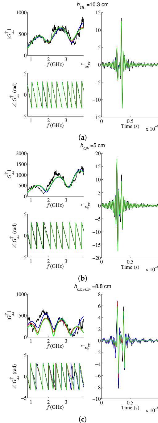
Figure 3. Measured (black curves) and modeled Green's functions in the frequency and the time domains for selected litter thickness levels of the (a) OL, (b) OF and (c) OL-OF configurations of the controlled experiment. The blue curves correspond to modeled Green's functions for the model considering only frequency dependence of litter effective electrical conductivity, reported by André et al. [33], the red curves represent modeled Green's functions for the model accounting for both surface roughness and frequency dependence of litter effective electrical conductivity, and the green curves are modeled Green's functions for the model considering surface roughness only.
