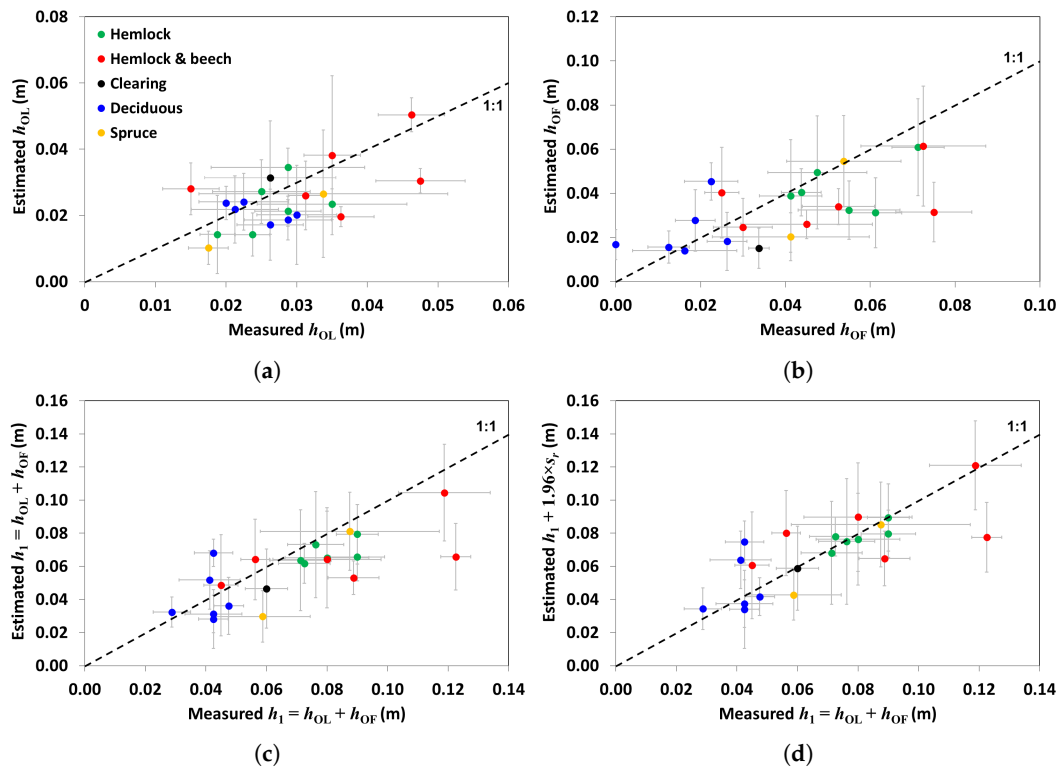
Figure 7. Comparison of inversion estimates for (a) OL litter layer thickness h_{OL} , for (b) OF litter layer thickness h_{OF} and for (c) total litter thickness h_1 with corresponding measured values, and of (d) total litter thickness estimates corrected by surface roughness coefficient ( h_1 + 1.96 \times s_r ) with measured total litter thickness, for the in situ experiment. The OL-OF litter configuration (see Figure 1c) is considered. Marker colors specify stand composition at each measurement location. Vertical and horizontal error bars represent 95% confidence intervals for the six estimated values and for the four measured values at each location, respectively. The dashed line is the 1:1 line.
