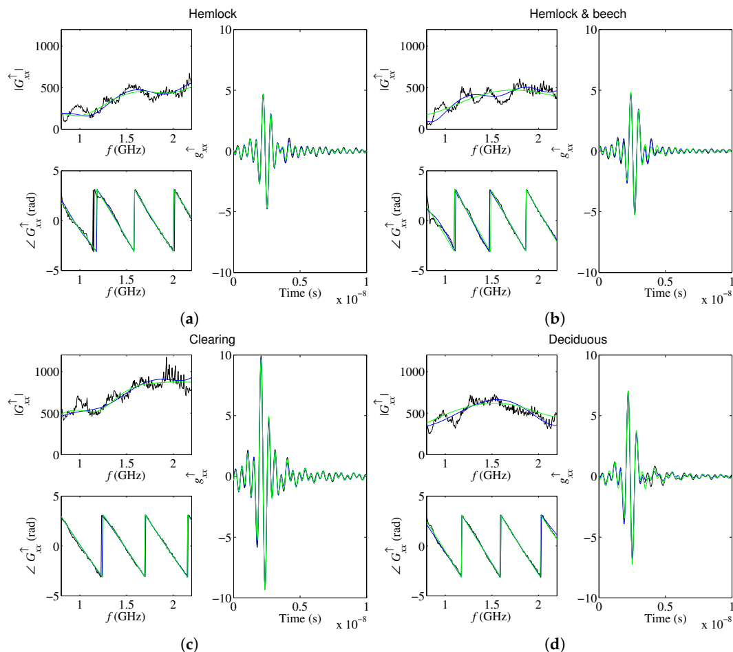
Figure 4. Measured (black curves) and modeled Green's functions in the frequency and the time domains for four contrasted situations of the in situ experiment: (a) litter of pure hemlock stand, (b) litter of mixed hemlock-beech stand, (c) litter in the clearing and (d) litter of the mixed deciduous stand. The blue curves represent the modeled Green's functions for the model considering only frequency dependence of litter effective electrical conductivity, reported by André et al. [34], and the green curves are the modeled Green's functions for the model accounting for surface roughness only.
