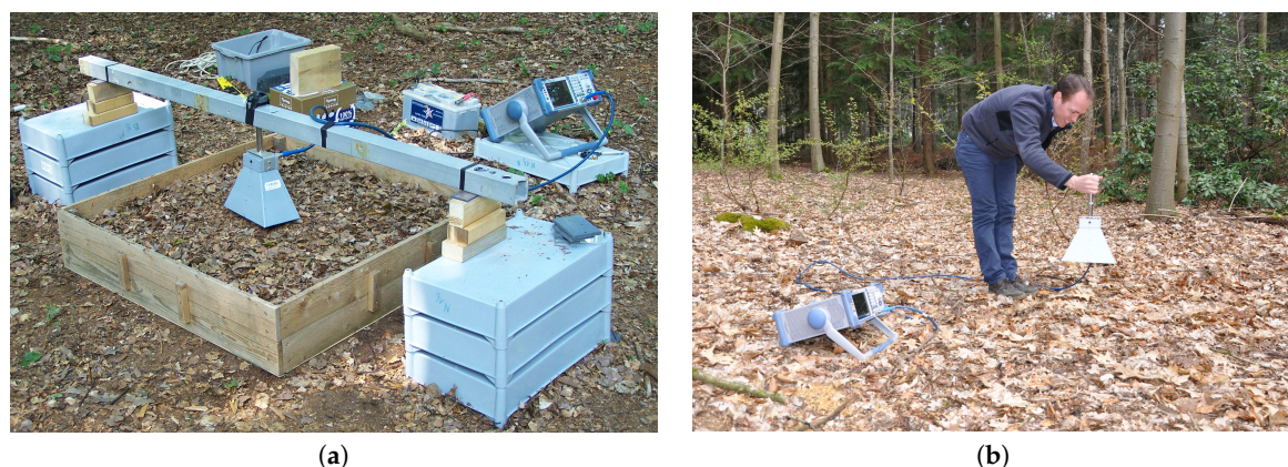
Figure 2. Pictures of the experimental setups for the (a) controlled (from [33]) and (b) in situ experiments.
