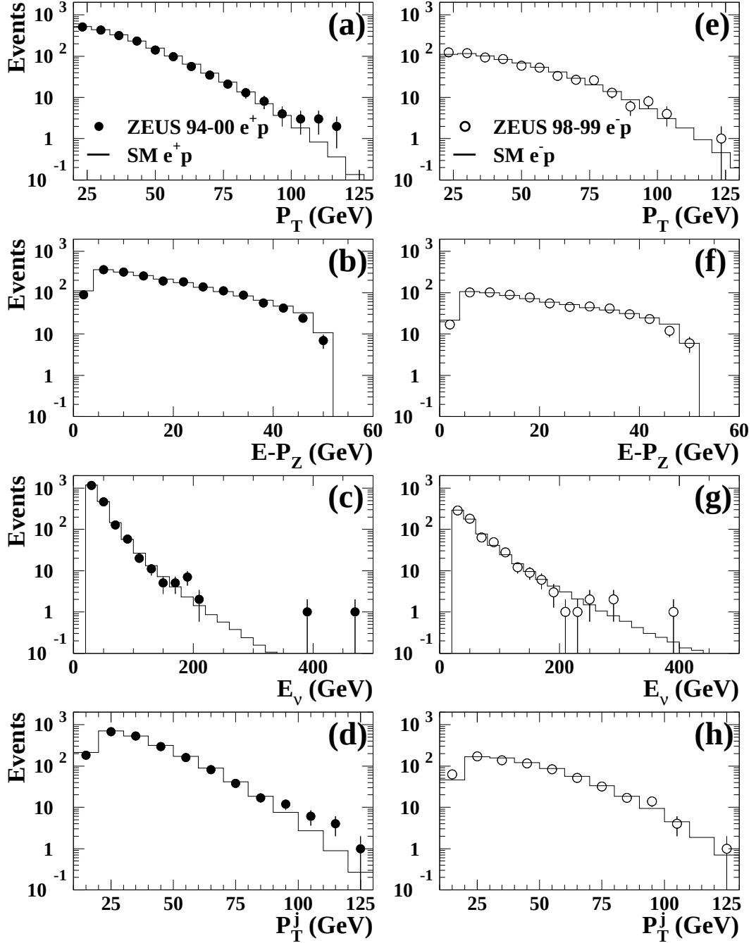
Figure 5: Comparison of distributions from 94-00 e^+p (a-d) and from 98-99 e^-p data sets (e-h) with the corresponding CC MC samples for the selected distributions: (a,e) missing transverse energy, P_T ; (b,f) E - P_Z ; (c,g) neutrino energy, E_\nu , and (d,h) jet transverse momentum, P_T^j .
