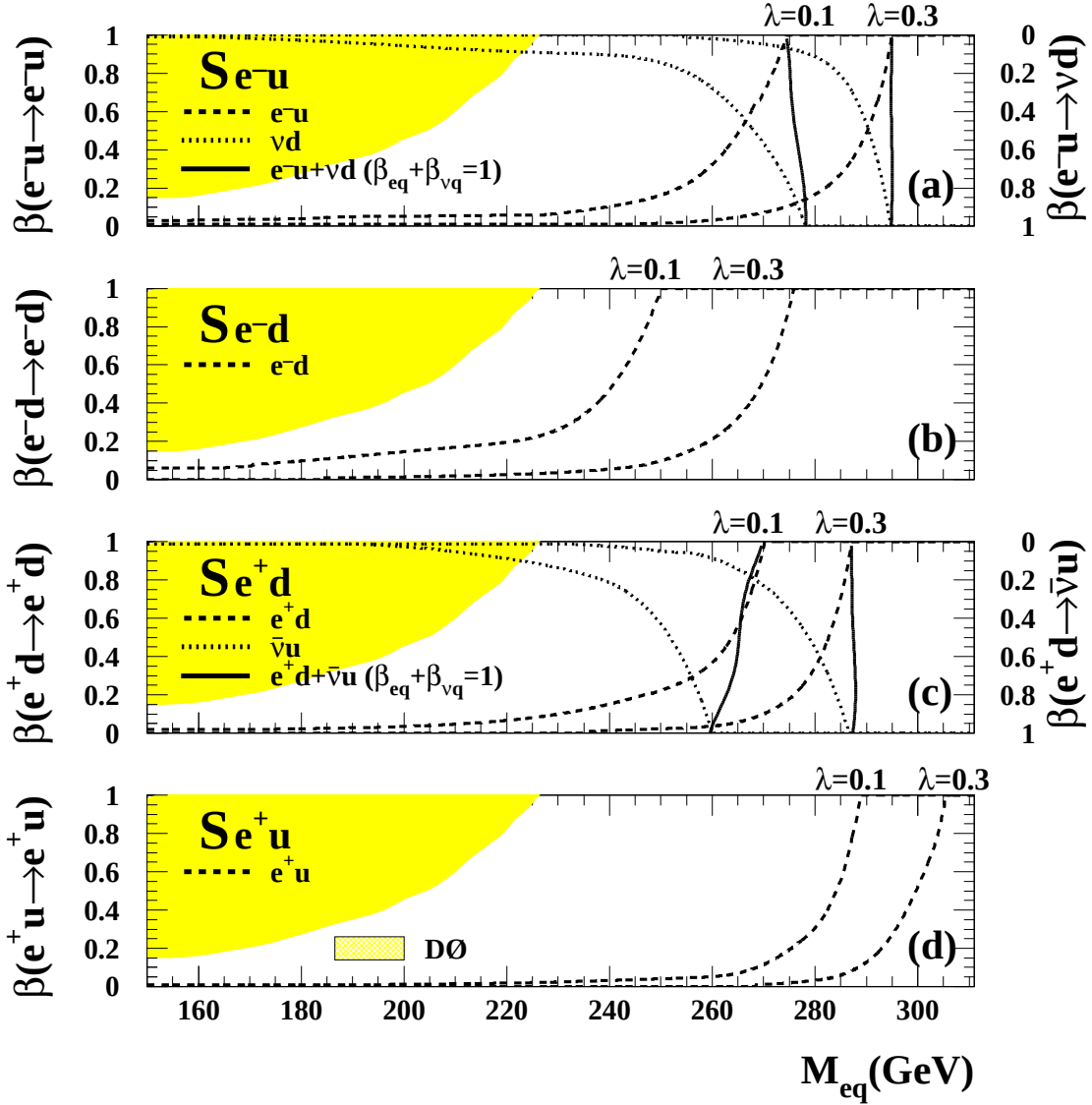
Figure 8: The constant- \lambda limits as a function of the branching ratios into eq and \nu q (shown on the left and right axes, respectively), and of the resonance mass ( x axes), for the scalar resonant states listed in Table 4. The dotted line corresponds to limits set with only the ep \rightarrow \nu X data set, the dashed line with only the ep \rightarrow eX data set; the solid black line is the limit set using both data sets, assuming \beta_{eq} + \beta_{\nu q} = 1 . For each limit curve, the area to the left of the curve is the excluded region. Results for the resonant states are shown for constant limit of \lambda = 0.1 and \lambda = 0.3 . The shaded area in each plot shows the area excluded by the D\bar{O} experiment.
