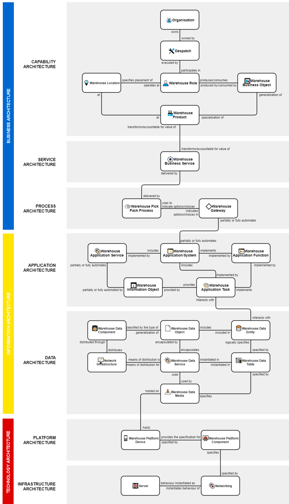
Fig. 1. Warehouse pick pack metamodel (from LEAD ID#-ES20001ALL)
