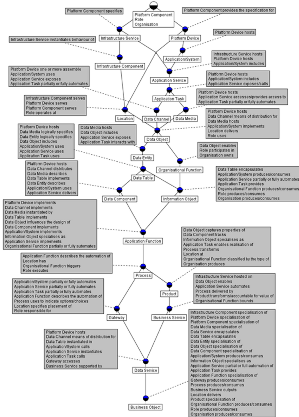
Fig. 3. 25ActiveInfrastructureService lattice
