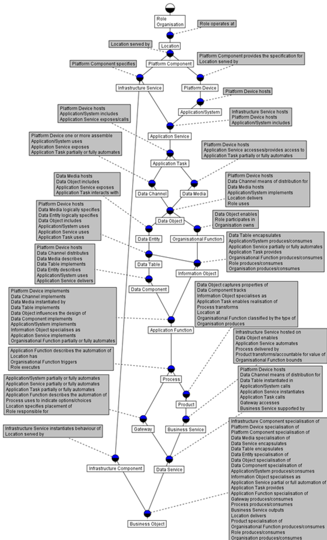
Fig. 4. 25v2ActiveInfrastructureService lattice
