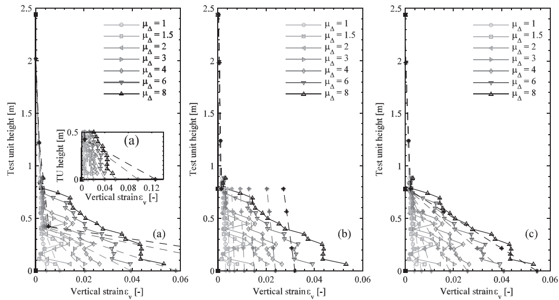
Figure 10. Experimental versus numerical vertical strain profiles of rebar N3 for test T9 at positive ductility levels: (a) FB 5 IPs, (b) two-element DB/c and (c) two-element DB/ae models.
