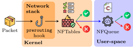
Fig. 4: General NFTables/NFQueue firewall operation
