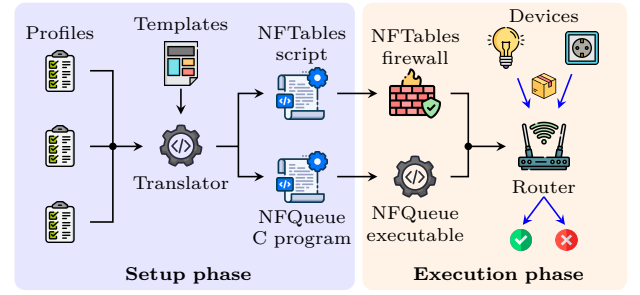
Fig. 2: System components
