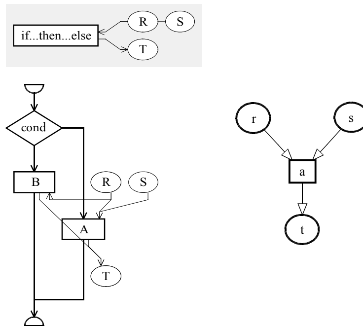
Figure 4.7 A standard alternative
