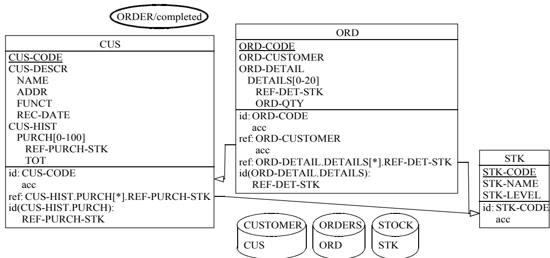
Figure 11.35 The refined physical schema
