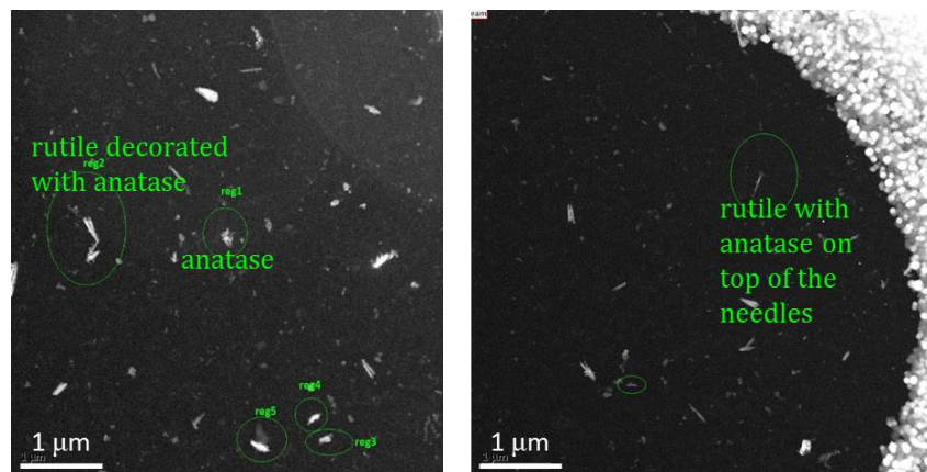
Figure 3-9: Global observation of one window of the grid, crystallites phases are attributed to anatase or rutile \text{TiO}_2 depending on their morphology.
