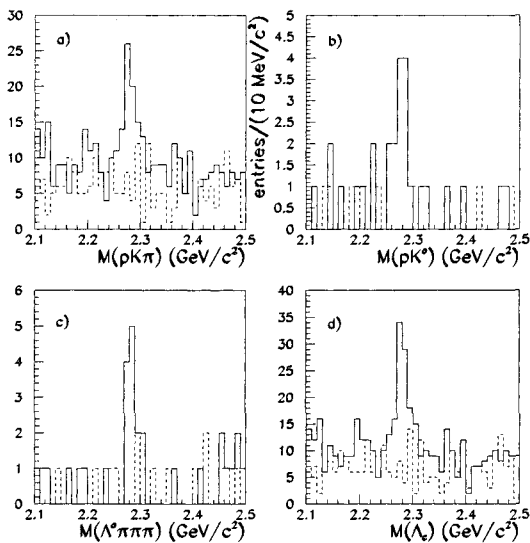
Fig. 7. Invariant mass distributions for right sign (full line) and wrong sign (dashed line) \Lambda_c candidates correlated with a high p_T lepton: a) pK\pi channel, b) pK^0 channel, c) \Lambda^0\pi\pi\pi channel, d) all channels combined
