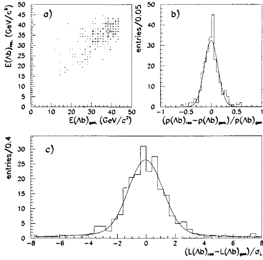
Fig. 3. a) Reconstructed vs generated b -baryon energy and b) distribution of the difference between reconstructed and generated momentum, normalised to the generated momentum, in the simulation sample; c) pull distribution for the reconstructed position of the b -baryon in the plane transverse to the beam direction. The curves in b) and c) represent the results of a Gaussian and a double Gaussian fit respectively to the distributions
