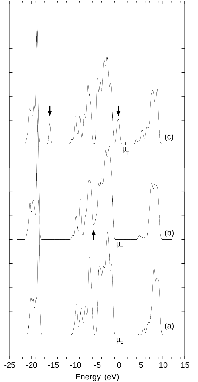
FIG. 7. Electronic density of states for (a) bulk \alpha -quartz, (b) the dense surface, and, (c) the cleaved surface. The fermi-level for the bulk \alpha -quartz and for the dense surface are aligned ( \mu_F=0 eV), the one of the cleaved surface has been shifted \mu_F=1.5 eV, in order to facilitate the comparison between the different parts.
