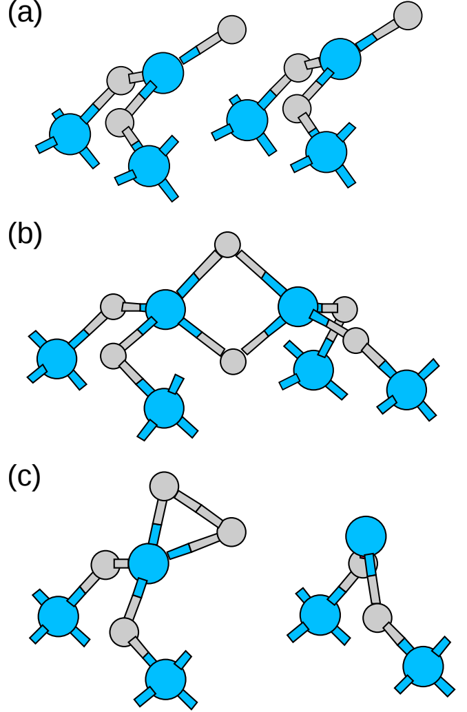
FIG. 1. Side view of (a) the cleaved surface, (b) an hypothetical 2 \times 1 reconstruction with edge-sharing tetrahedra, and (c) the dimer surface. Si and O atoms are represented in dark and pale grey, respectively.
