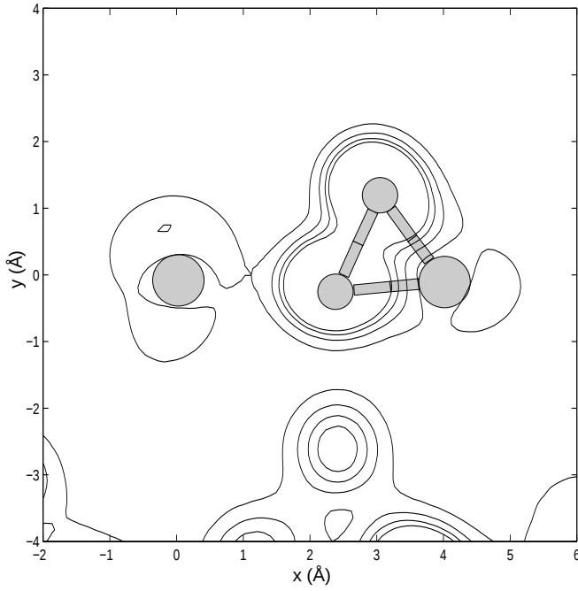
FIG. 2. Contour plot of the electronic density on the oxygen-dimer at the dimer surface. The contour is drawn in a plane passing through the Si atom with the dimer, the 2-coordinated Si, and the lower oxygen of the dimer. Note that the upper oxygen is almost co-planar with these atoms. The x axis is defined by the 2 silicons. The origin of the x and y axis (defined by orthogonality with x ) is the 2-coordinated Si. As a guide for the eyes to locate the atoms, we superimposed (in pale grey) to the contour plot a ball and stick representation of the structure: the big circles are Si atoms while the small ones are O atoms. The oxygen dimer clearly appears at the center of the picture, while the electronic density is increased on the 2-coordinated silicon with respect to 4-coordinated silicons. At the bottom of the figure, there is another peak of density. It corresponds to an oxygen located just above the dimer which repels it towards the outside. The contour interval is 0.5 \text{ e}^-/\text{\AA}^3 .
