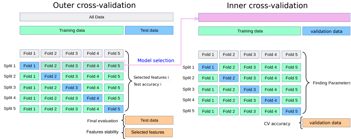
Fig. 1 Overview of the proposed method. The figure represents the nested 5-fold CV subsampling of the entire dataset, i.e., top-left gray bar. (Left) The outer CV is used to evaluate the performance of the model. The 80% of the data, i.e., four folds (pink box), is used as training set, where the best model and features are selected. The remaining 20% is used as testing set, to evaluate the performance of the model. (Right) Within the inner CV, four folds are used for training and the hold-out fold as validation set. The best model, features and parameters are selected according with the best CV accuracy. The outer CV is shuffled 20 times, generating 100 subsamplings of the dataset and therefore the same number of selected features 'fingerprints'. The stability of selected biomarkers and the final accuracy is assessed over all subsampling estimations.
