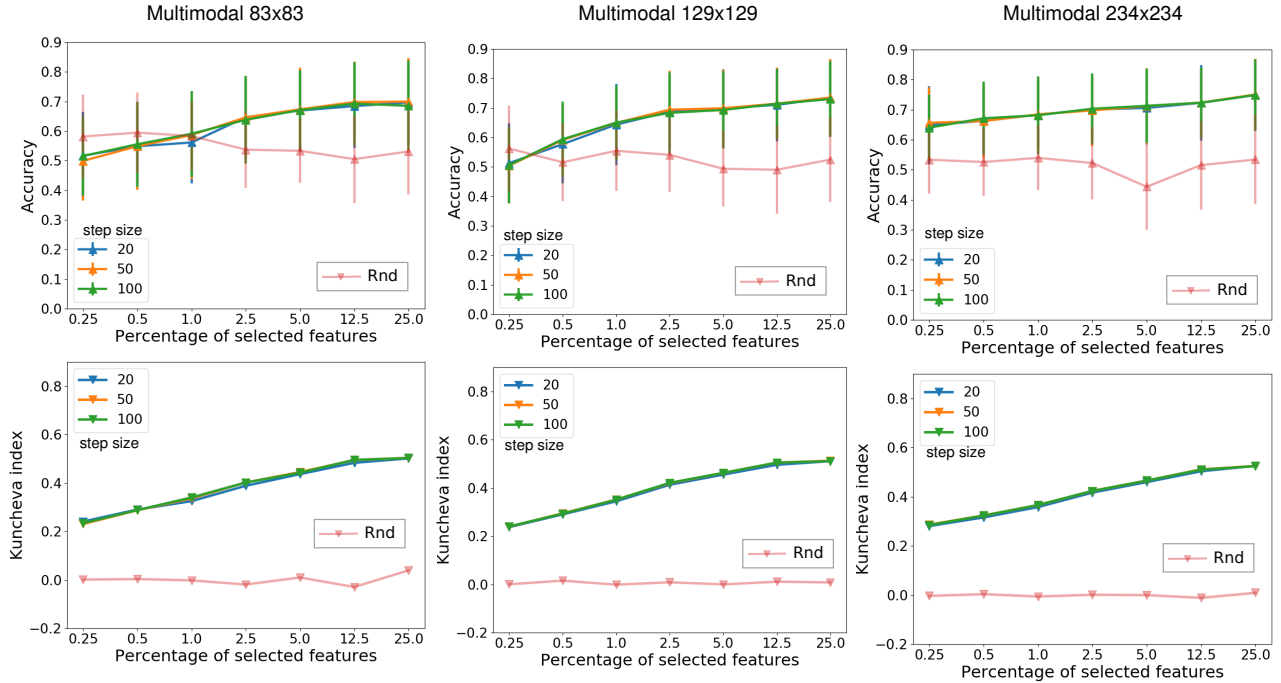
Fig. 5 Each column represents the mean accuracy of the outer CV folds \pm standard deviation (top) and stability (bottom) for a given scale of the multimodal connectome. The step size corresponds to the percentage of features dropped at each step of the RFE-SVM algorithm. Red curve represents a random selection of features.
