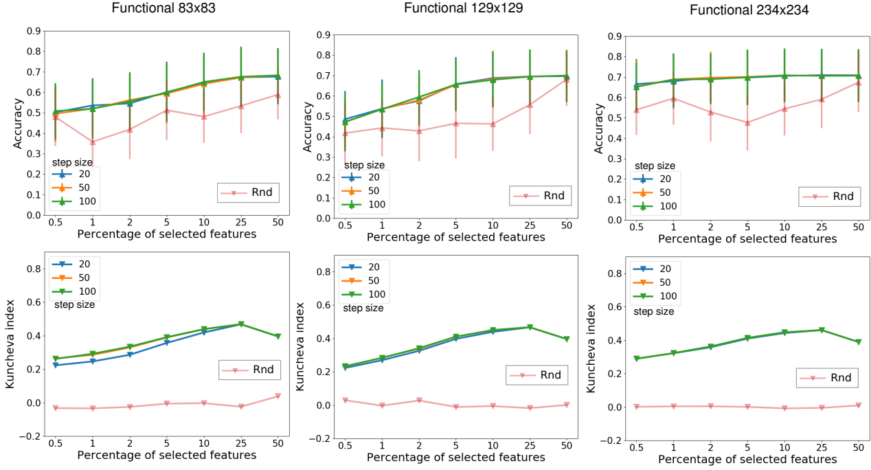
Fig. 4 Each column represents the mean accuracy of the outer CV folds \pm standard deviation (top) and stability (bottom) for a given scale of the functional connectome. The step size corresponds to the percentage of features dropped at each step of the RFE-SVM algorithm. Red curve represents a random selection of features.
