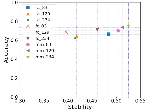
Fig. 3 Best accuracy versus stability for all considered modalities and resolutions.
