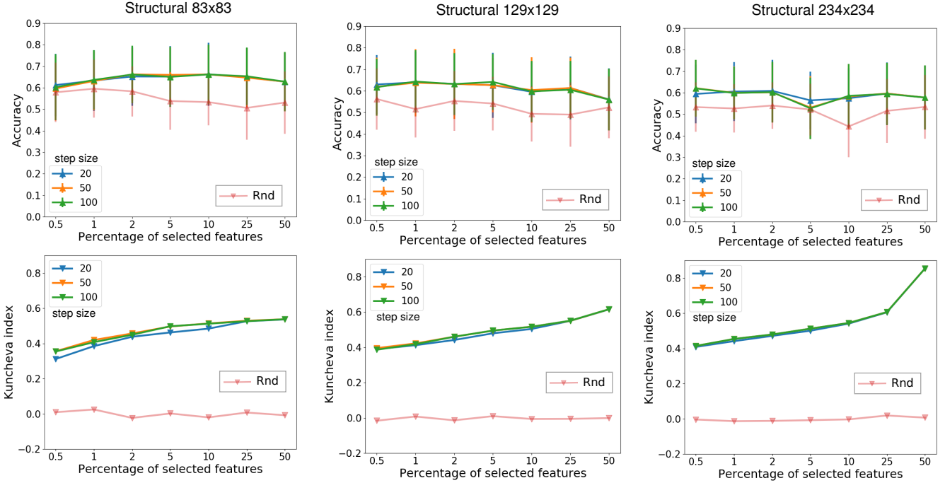
Fig. 2 Each column represents the mean accuracy of the outer CV folds \pm standard deviation (top) and stability (bottom) for a given scale of the structural connectome. The step size corresponds to the percentage of features dropped at each step of the RFE-SVM algorithm. Red curve represents a random selection of features.
