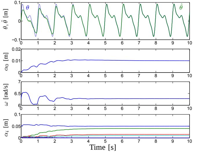
Fig. 4. Signal learning by an adaptive oscillator containing 8 harmonics. After 3 seconds, the state variables have converged to the actual features of the input signal. As expected, only 4 amplitudes converged to non-zero values, since the input signal contained only 4 harmonics (+ offset).
