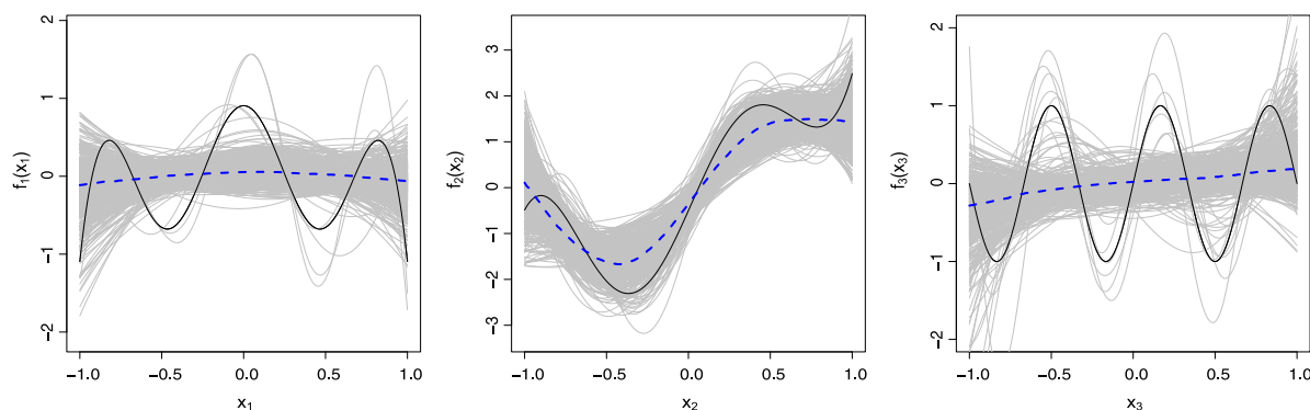
Fig. 2. Estimation of smooth additive terms (gray curves) for S = 500 dataset replications of size n = 300 in the Bernoulli scenario with LPS. The dashed line is the pointwise median of the gray curves and the black curves are the target functions.
