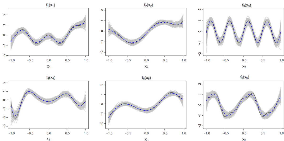
Fig. 4. Estimation of smooth additive terms f_1, \dots, f_6 (gray curves) for S = 500 dataset replications of size n = 300 in the Binomial scenario. The dashed line is the pointwise median of the gray curves.
