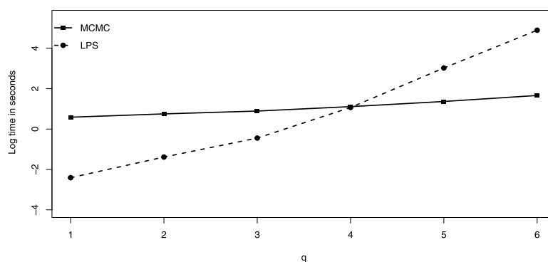
Fig. 5. Logarithm of the average computation time (in seconds) of LPS (dashed) and LPS-MCMC (solid) over S = 20 samples of size n = 300 and dimensions q \in \{1, 2, 3, 4, 5, 6\} .
