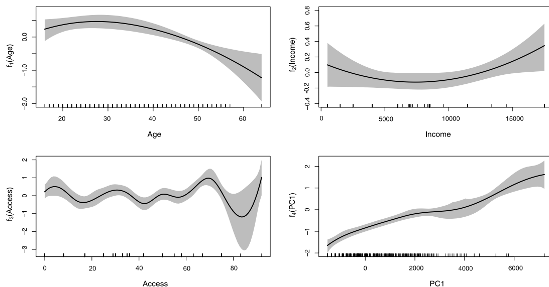
Fig. 6. Estimated smooth functions (solid curve) and 95% approximate pointwise credible intervals (gray surface) for variables Age , Income , Access and PC1 .
