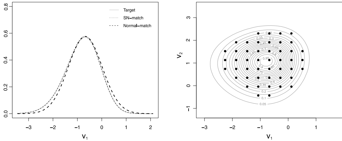
Fig. 1. Left: Skew-normal fit (dotted) and naive Gaussian match (dashed) to the conditional \tilde{p}(v_1|\hat{v}_2, \mathcal{D}) (gray). The skew-normal fit is closer to the target and captures the lack of symmetry present in the target. Right: Final grid construction to explore \tilde{p}(\mathbf{v}|\mathcal{D}) .
