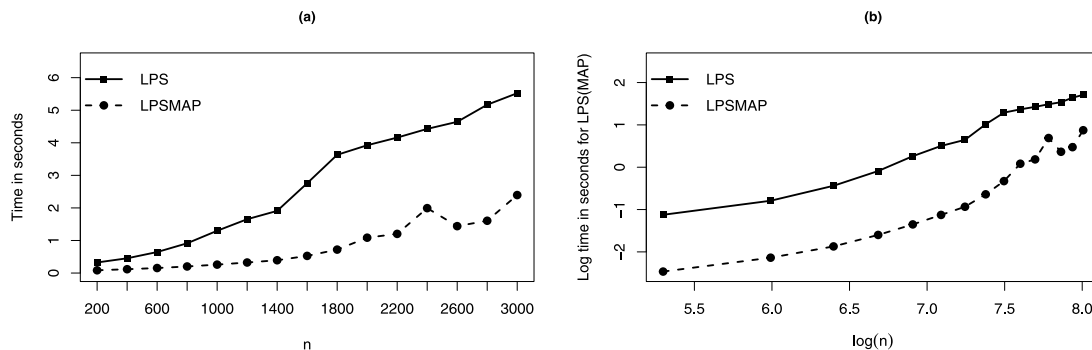
Fig. 3. (a) Real elapsed time in seconds as a function of sample size for LPS and LPSMAP. (b) Log of computational time (in seconds) of LPS(MAP) against log sample size.
