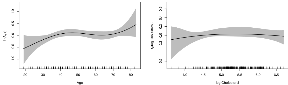
Fig. 7. Estimated smooth functions (solid curve) and 95% approximate pointwise credible intervals (gray surface) for variables Age and log(Cholesterol) of the nutritional study dataset.
