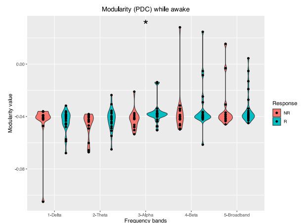
Figure 6: Modularity from PDC binarized thresholded data in awake condition. *: p-value \leq 0.05 .
