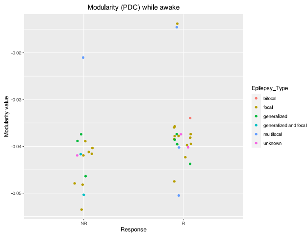
Figure 9: Modularity on Alpha band derived from PDC connectome in awake condition, grouped by therapy response and clustered by epilepsy type.
