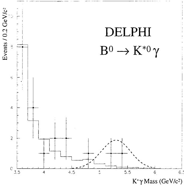
Fig. 4. The mass distribution for the (K^+\pi^-)_{K^{*0}\gamma} system. Points with error bars represent the real data and the histograms the expected mass distributions in the absence of charmless radiative B decays, as obtained from simulation. The dashed curve represents the expected B^0 \rightarrow K^{*0}\gamma signal corresponding to the 90 % upper limit quoted
