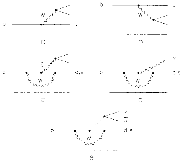
Fig. 1. Feynman diagrams of the main processes contributing to the rare b decays studied in the present paper: hadronic charmless b decays through tree level diagrams (a and b) and penguin diagrams (c), and radiative (d) and dineutrino (e) decays also through penguin diagrams
