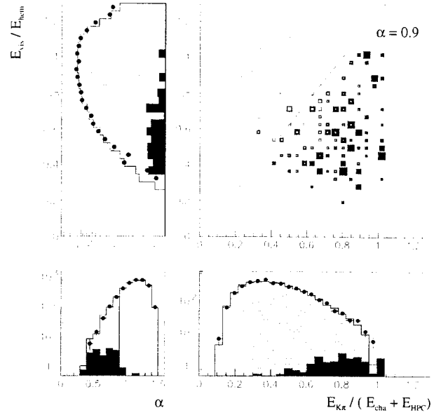
Fig. 5. Distributions for the E_{vis} / E_{hem} (upper left) and E_{K\pi} / (E_{cha} + E_{HPC}) (lower right) variables used in the search for dineutrino charmless B decays and their correlation (upper right). The angular variable \alpha used to select the signal enriched region is shown in the lower left plot. The cut \alpha = 0.9 is also shown (upper right and lower left). Real data are shown by the closed circles, the background from simulation by the light grey histograms, and the distributions expected for signal B \rightarrow K^*\nu\bar{\nu} events by the dark grey histograms
