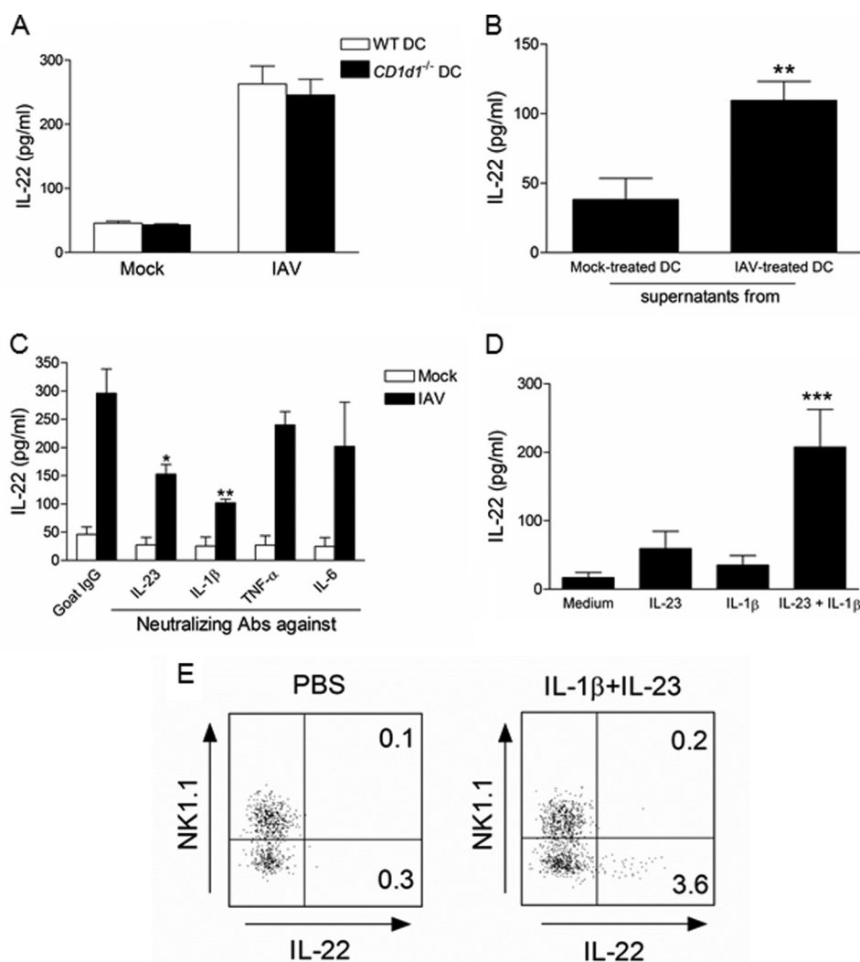
FIGURE 5. Mechanisms involved in IAV-induced IL-22 release by NK1.1 neg iNKT cells. A, IAV-infected WT or CD1d1 -/- DCs were cultured with sorted liver iNKT cells. Of note, in response to the canonical iNKT cell agonist \alpha -galactosylceramide, CD1d deficiency in DC fully abrogated IFN- \gamma production by iNKT cells (data not shown). B, after 16 h, undiluted supernatant from mock-treated or IAV-infected DCs was added to iNKT cells. C, IAV-infected DCs were cultured with iNKT cells in the presence of neutralizing anti-IL-23, anti-IL-1 \beta , anti-TNF- \alpha , anti-IL-6, or isotype control mAbs (5 \mu g/ml). D, purified iNKT cells were incubated with recombinant IL-23 and/or IL-1 \beta protein(s) (1 ng/ml). Of note, TNF- \alpha and IL-6 were without effect on IL-22 release (data not shown). A–D, two days later, IL-22 production was measured by ELISA. Data represent the mean \pm S.D. of at least three independent experiments performed in triplicate. B, differences in mean were analyzed using the two-tailed Student's t test. **, p < 0.01. C and D, a one-way ANOVA was used to analyze the variance followed by a Bonferroni multiple comparison test to compare all groups. *, p < 0.05; **, p < 0.01; ***, p < 0.001. E, shown is intracellular staining of IL-22 in lung iNKT cells. Lung mononuclear cells treated with IL-1 \beta and IL-23 (10 ng/ml) for 4 h in the presence of brefeldin A and gated iNKT cells expressing or not the NK1.1 marker were analyzed for intracellular IL-22 production. Gates were set based on the isotype control. The percentage of iNKT cells expressing IL-22 is shown. One representative experiment of two is depicted.
