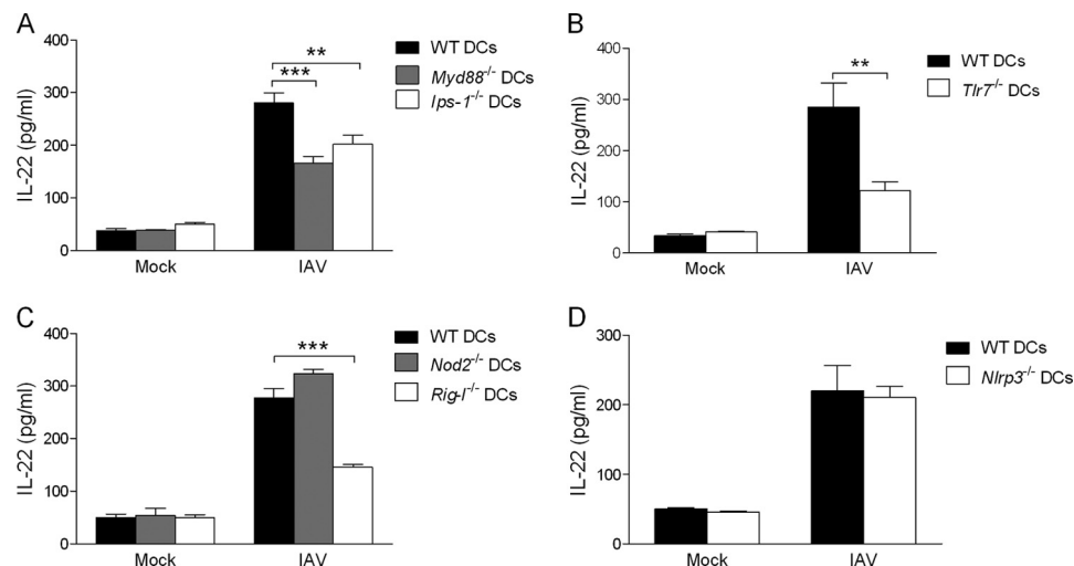
FIGURE 4. Role of innate sensors in IL-22 release by iNKT cells. WT, Myd88 -/- and Ips-1 -/- (panel A), WT and Tlr7 -/- (panel B), WT, Nod2 -/- , and Rig-I -/- (panel C), or WT and Nlrp3 -/- (panel D) DCs were exposed or not (mock) to IAV (m.o.i. = 1) for 16 h, extensively washed, and co-cultured for 48 h with purified liver iNKT cells. Cytokine production was quantified by ELISA. Data represent the mean \pm S.E. of at least three independent experiments performed in triplicate. A–C, a one-way ANOVA has been used to analyze the variance followed by a Bonferroni multiple comparison test to compare all groups. **, p < 0.01 ; ***, p < 0.001 . B–D, differences in mean were analyzed using the two-tailed Student's t tests. **, p < 0.01 .
