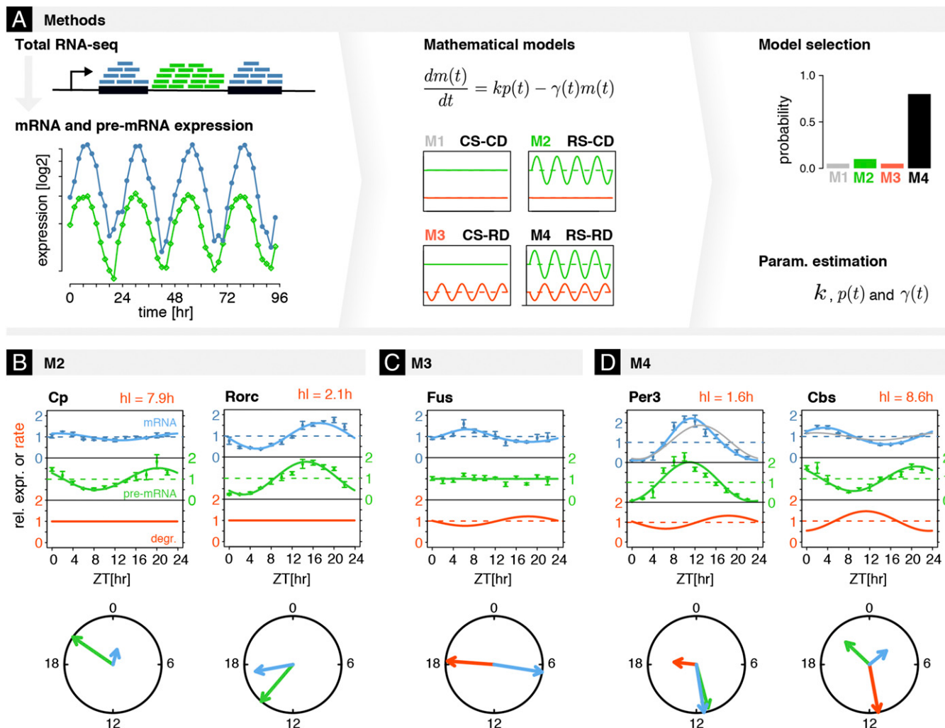
Fig. 1. Kinetic model identifies contributions and parameters of rhythmic transcription and rhythmic degradation regulating mRNAs from total RNA-seq. (A) Temporal accumulations of mRNA and pre-mRNA from time-resolved total RNA-seq were used to fit four kinetic models (M1–M4). The rate equation for the temporal accumulation of mRNA m(t) depends on pre-mRNA p(t) and the degradation rate \gamma(t) , which are either constant or parameterized with periodic functions ( Materials and Methods ). The models allow for constant (C) or rhythmic (R) synthesis (S) and degradation (D) in the four combinations: M1 (constant synthesis and constant degradation, CS-CD), M2 (rhythmic synthesis and constant degradation, RS-CD), M3 (constant synthesis and rhythmic degradation, CS-RD), and M4 (rhythmic synthesis and rhythmic degradation, RS-RD). Probabilities for each model are estimated using Schwarz weights ( Materials and Methods ); the optimal model for each mRNA (one per gene; Materials and Methods ) also yields gene-specific parameters (e.g., mRNA half-life, processing time, phases, and amplitudes of rhythmic degradation rates). We applied this approach genome-wide. (B–D) Temporal profiles of mRNA and pre-mRNA of genes assigned to models M2–M4. Data for mRNA (blue) and pre-mRNA (green) with error bars (SE over four biological replicates) are shown as relative expression, that is, the total normalized counts divided by the average value over time. Solid curves are the fitting for the optimal model and estimated parameters (blue, mRNA; green, pre-mRNA; red, degradation). Peak times (phase) and amplitudes are summarized in circle plots. The radial scale of these plots is relative to the largest relative amplitude of mRNA, pre-mRNA, or rhythmic degradation. Absolute half-lives [ \log(2)/\gamma_0 , in hours], if identifiable, are labeled. (B) M2: (Left) Cp had long estimated hl (7.9 h), which damped amplitude of mRNA compared with that of pre-mRNA; (Right) Rorc mRNA was identified in M2 (RS-CD) with estimated constant hl of 2.1 h. (C) M3: Fus mRNA was identified in M3 (CS-RD). The peak time of rhythmic degradation (RD) was ZT18.3 and the relative amplitude of RD was 0.3. Mean half-life was nonidentifiable ( Materials and Methods ). (D) M4: (Left) Per3 mRNA was identified in M4 (RS-RD). The RD showed a maximum at ~ZT18, and a relative amplitude of 0.5 mean degradation rate was identifiable with mean hl of 1.6 h; (Right) Cbs mRNA showed a phase delay between mRNA and pre-mRNA > 6 h, which could be explained by M4. Parameters of RD showed a maximum at ~ZT9 with a mean hl of 8.6 h.
