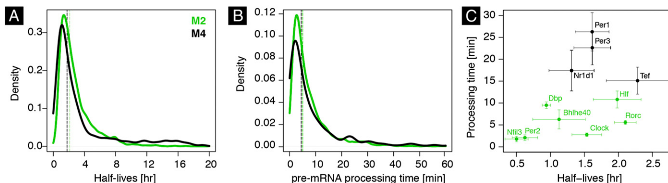
Fig. 3. Distributions of estimated half-lives and processing times of mRNA in mouse liver. (A) Distribution of estimated mRNA half-lives [ \log(2)/\gamma_0 , in hours] in M2 and M4 for transcripts with identifiable half-lives. Vertical lines indicate the medians of the distributions. (B) Distribution of pre-mRNA processing times ( 1/k , in minutes) in models M2 and M4. Vertical lines indicate the medians of the distributions for transcripts with identifiable parameters. (C) Half-lives and processing times of core clock and clock output mRNAs. We plotted standard errors (SEs) of the estimates when available ( SI Materials and Methods and Dataset S1 ).
