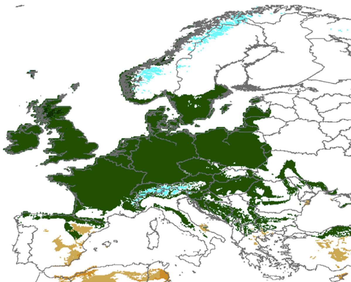
Figure 4: Occurrence of Köppen–Geiger climate types BSh, BSk, Cfb, Cfc and ET in Europe (Source: EFSA PLH Panel, 2020)
