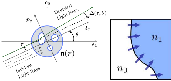
Fig. 5: (left) Model of light deflection through a transparent object. (right) TV model of RIM. Fig. 6: An example of RIM reconstruction for a bundle of fibres with (left) the FBP and (right) TV minimization approach.
