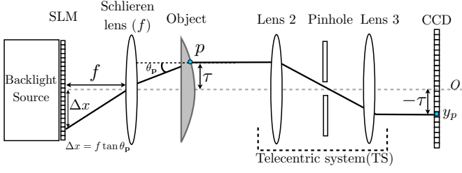
Fig. 2: A 2-D schematic of Schlieren deflectometer.
