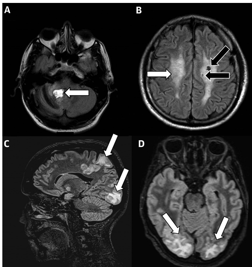
FIGURE 2 Brain MRI
