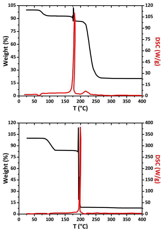
Fig. 4. TG (black) and DSC (red) analyses for 1 (top) and 2 (bottom). (For interpretation of the references to colour in this figure legend, the reader is referred to the web version of this article.)
