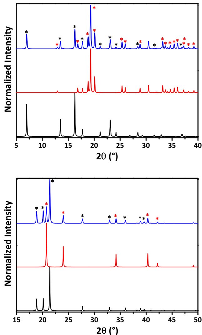
Fig. 5. Experimental (blue) X-ray powder diffraction patterns of final residues obtained after TG analyses of 1 (top) and 2 (bottom). Calculated for \text{CoCl}_2 (black) and \text{Co}_2\text{N} (red) X-ray powder diffraction patterns (top). Calculated for hexagonal (black) and cubic (red) X-ray powder diffraction patterns of elemental cobalt (bottom). (For interpretation of the references to colour in this figure legend, the reader is referred to the web version of this article.)
