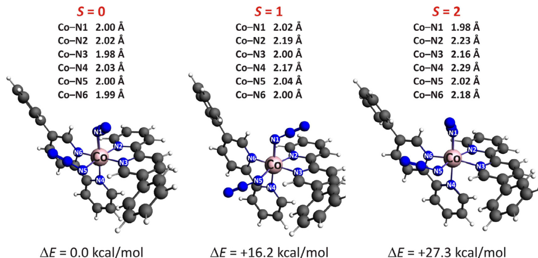
Fig. 6. The lowest energy conformations of the cobalt(III) complexes [\text{CoL}_2(\text{N}_3)_2]^+ , characterized by various spin states based on the ADF/BLYP-D3/TZP calculations.
