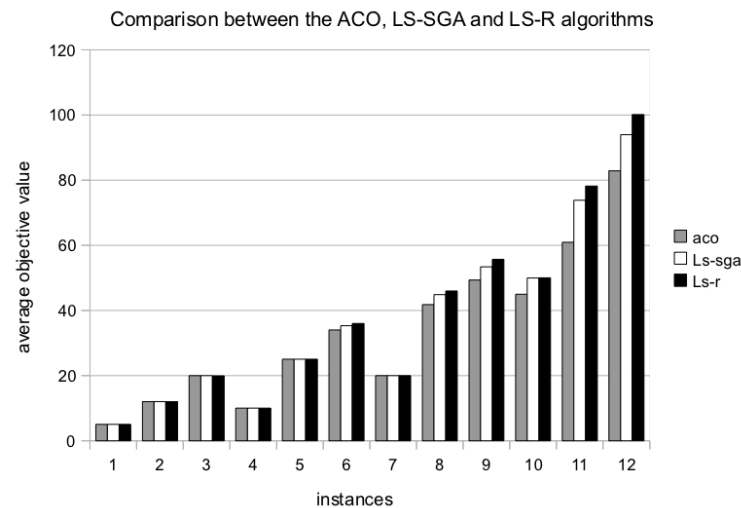
Figure 5.26: Comparison between the ACO, LS-SGA and LS-R algorithms on planar instances
