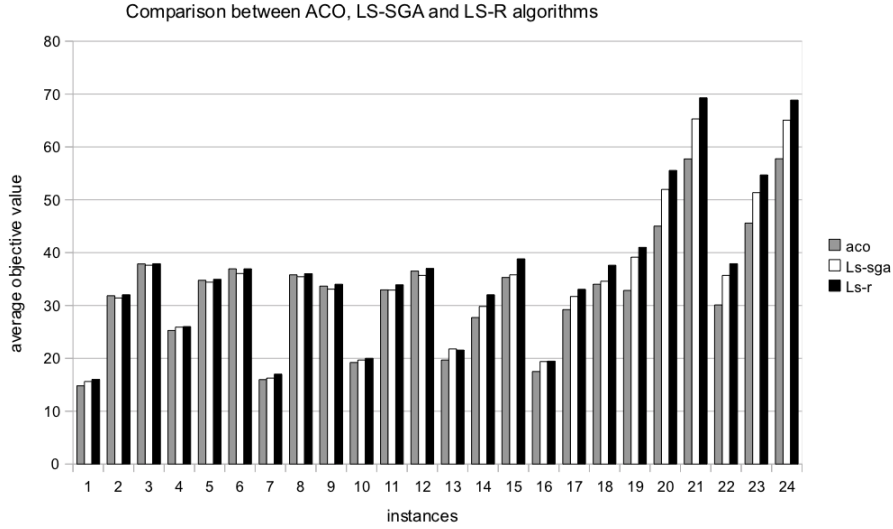
Figure 5.24: Comparison between the ACO, LS-SGA and LS-R algorithms on mess instances
