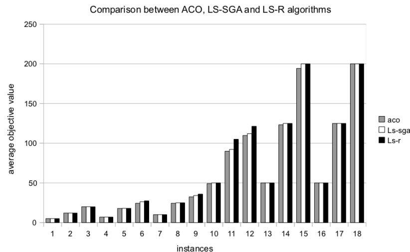
Figure 5.25: Comparison between the ACO, LS-SGA and LS-R algorithms on steiner instances
