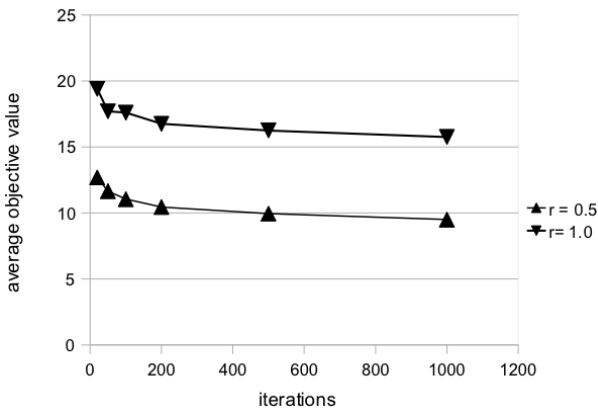
Figure 5.36: Grid 15x15: average objective value over iterations
