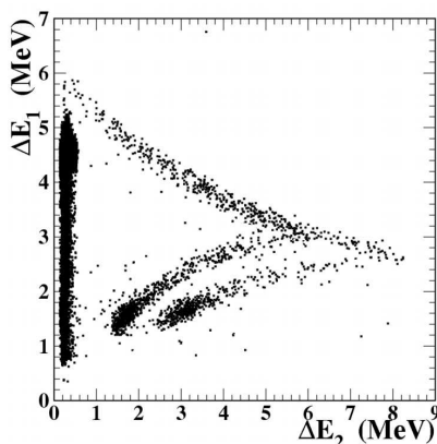
FIG. 2.— \Delta E_1 - \Delta E_2 spectrum at a beam energy of 5.55 MeV on a 200 \mu\text{gr}/\text{cm}^2 (\text{CD}_2)_n target. The c.m. energy range covered is 1.0 to 1.23 MeV.
