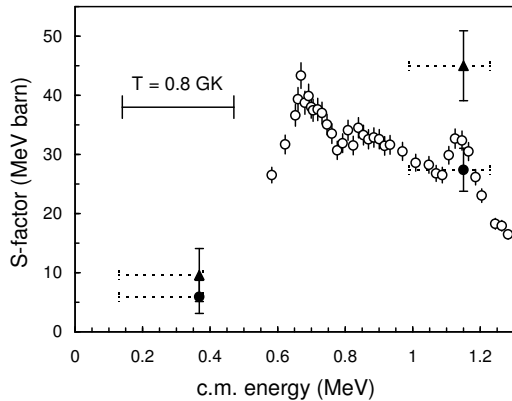
FIG. 4.— Astrophysical S factor of the {}^7\text{Be}(d,p){}^8\text{Be} reaction. Open circles: data from Kavanagh (1960); filled circles: present data including contributions from the ground and first excited states of {}^8\text{Be} only; filled triangles: total S -factor derived from the present experiment. The vertical error bars are the total error. The horizontal dotted bars indicate the energy range covered at each data point. The Gamow window for a typical BBN temperature T=0.8 GK is also shown.
