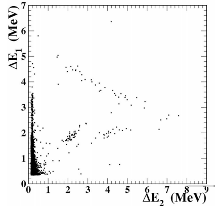
FIG. 3.— Same as Fig. 3 for a beam energy of 1.71 MeV, corresponding to a c.m. energy range of 0.13 to 0.38 MeV.
