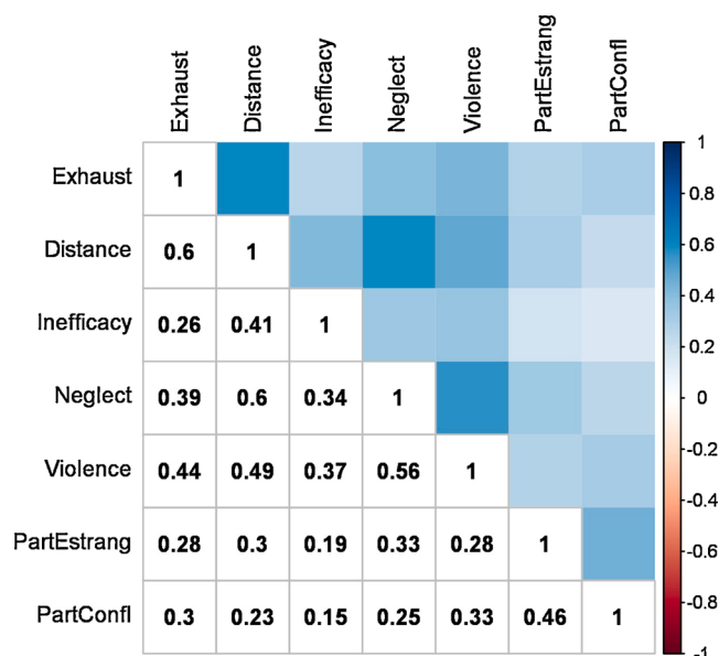
Fig. 1. Pearson product-moment correlations between each nonparanormal-transformed variable.
