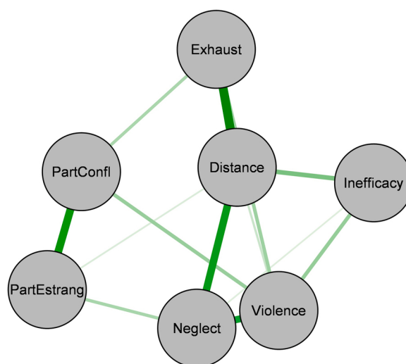
Fig. 2. Graphical Gaussian Model Network Constructed via the Graphical LASSO.
