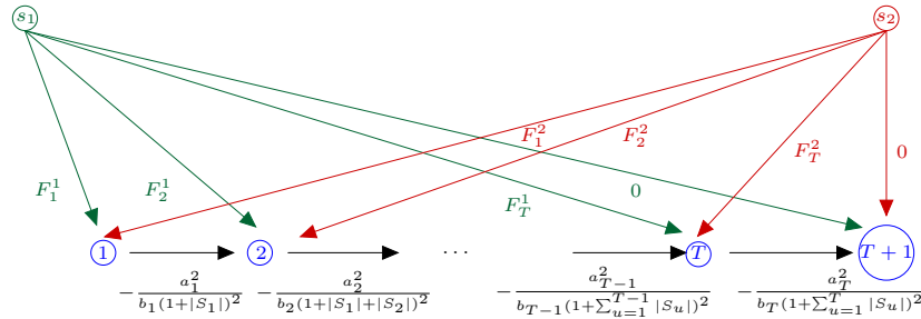
Figure 1: Congestion game for ULSG-sim with m = 2 .
