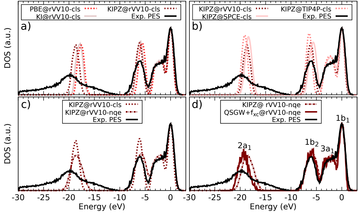
Figure 3: The density of states (DOS) obtained with the different methodologies are plotted and compared to the experimental photoemission spectra (PES). 82 All values are aligned and normalized by the 1b 1 peak.
